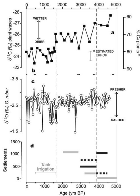
Figure 3. (a) \delta^{13}\text{C} plant wax record from core 16A as the weighted average of n -alkanoic acids \text{C}_{26} – \text{C}_{32} . Error bar represents the maximum propagated error ( 1\sigma error; see auxiliary material) in the estimate of % \text{C}_4 plant cover. Vertical black dashed lines identify steps in the aridification at ca. 4,000 and 1,700 years BP. (b) Calibrated radiocarbon ages ( 1\sigma error) in core 16A. (c) \delta^{18}\text{O} measured on Globigerinoides ruber from core 16A; values are corrected for ice volume effects. (d) Number of settlements based on archaeological data expressed as totals over culturally defined time intervals (see auxiliary material). In solid gray, sites from the Deccan Plateau (Andhra Pradesh, Karnataka, Maharashtra). In solid black, Indus (Harappan) sites from the dry Baluchistan, Sindh, Gujarat, Cholistan and lower Punjab. In dashed black, sites from rainier upper Punjab and Haryana. The drought-prone regime in the late Holocene (after 1,700 years BP) coincides with the flourishing of water tank construction.
