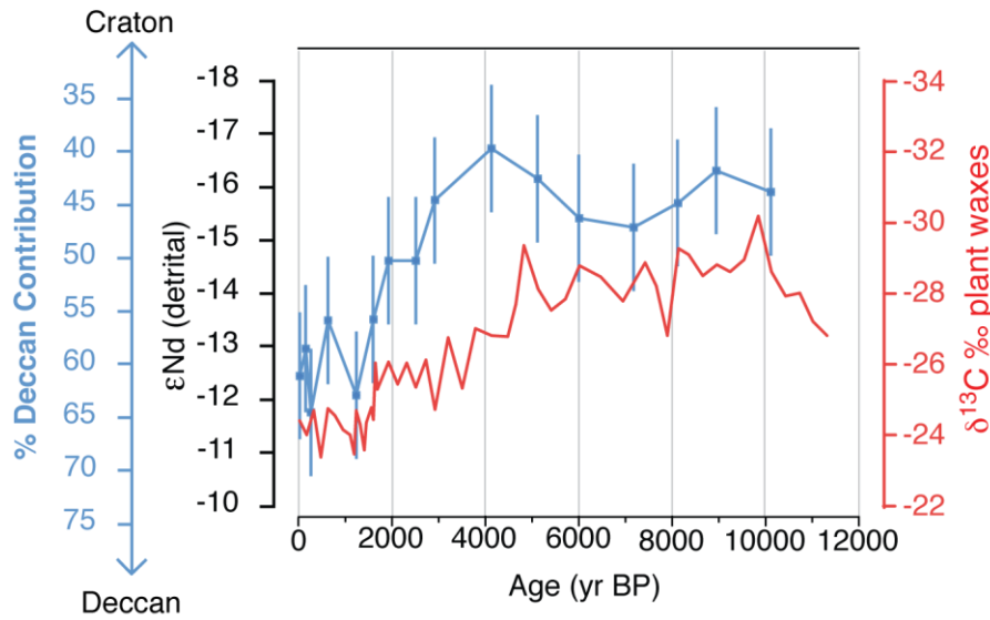
Figure 9. \epsilon Nd values in blue (provenance proxy) and \delta^{13}C_{wax} in red (proxy for aridity). Error bars on the \epsilon Nd curve apply only to the “% Deccan contribution” axis on the far left in blue, and result from an error propagation analysis based on the end-member \epsilon Nd estimates for the Deccan Plateau and the Indian craton.
