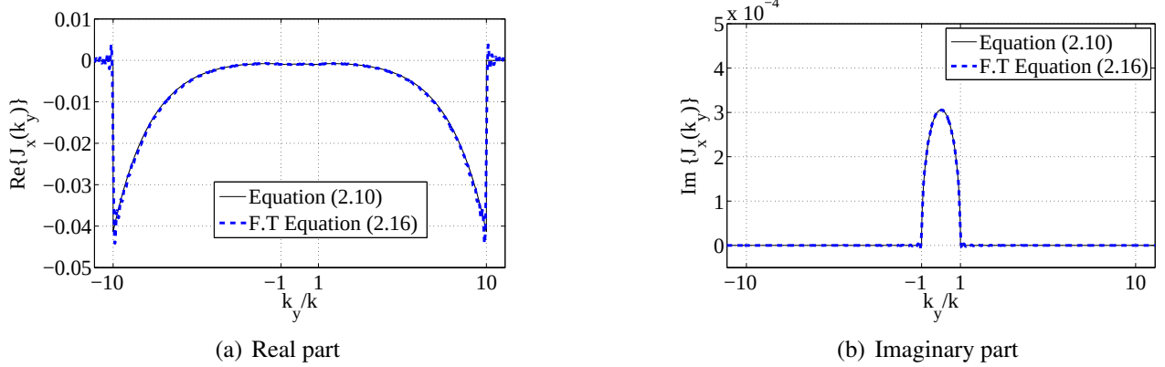
Figure 2.5: The (a) real and (b) imaginary parts of the spectral representation of the current density J_x(k_y) . The solid line represents Equation (2.10) and the dashed line represents the numerical Fourier transform of Equation (2.16) (form [13]).
