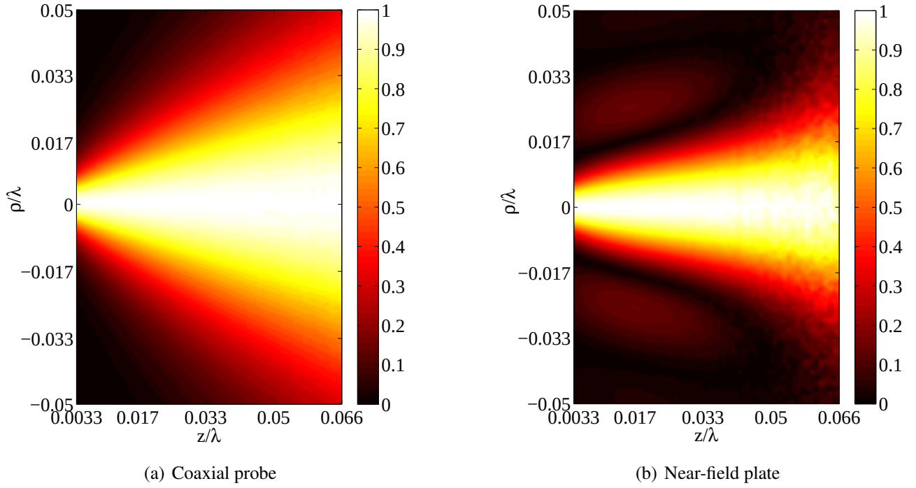
Figure 4.11: Measured beam emitted from (a) the coaxial probe and (b) the concentrically corrugated near-field plate. In both plots, the measured field along each z = z' plane is normalized to its maximum value: E_z(\rho, z = z')/E_z(\rho = 0, z = z') . The near-field patterns along z = 0.066\lambda = 20 mm, z = 0.05\lambda = 15 mm, and z = 0.033\lambda = 10 mm are plotted in Figure 4.8 (from [20]).
