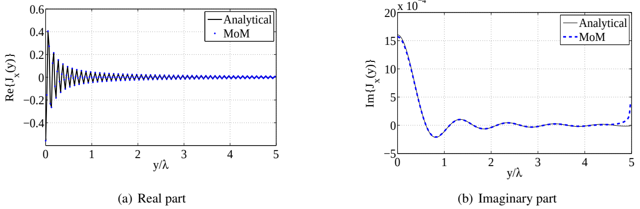
Figure 2.6: The (a) real and (b) imaginary parts of the current density J_x(y) . The solid line represents the analytically derived current density given by Equation (2.16). The dots in (a) and the dashed line in (b) represent the numerically (MoM) computed current density. The current density is only shown on half of the plate since it is symmetric about y = 0 (form [13]).
