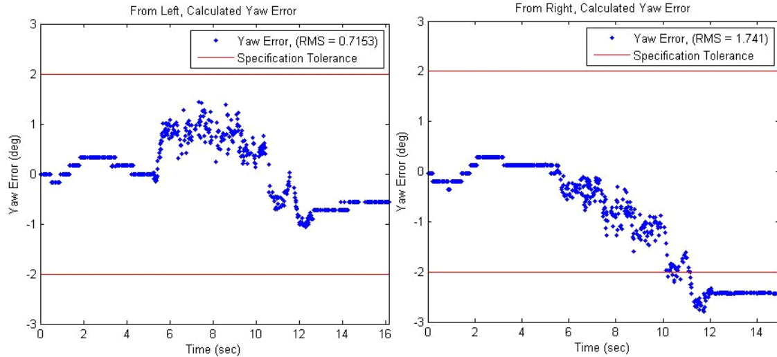
Figure 23. MTx yaw accuracy for the free swing medium reference angle test.
