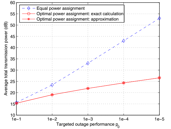
Fig. 10. Comparisons of the average total transmission power of the equal and optimal power assignment strategies with different targeted outage probabilities. L = 5 , \gamma_0 = 10 dB.
