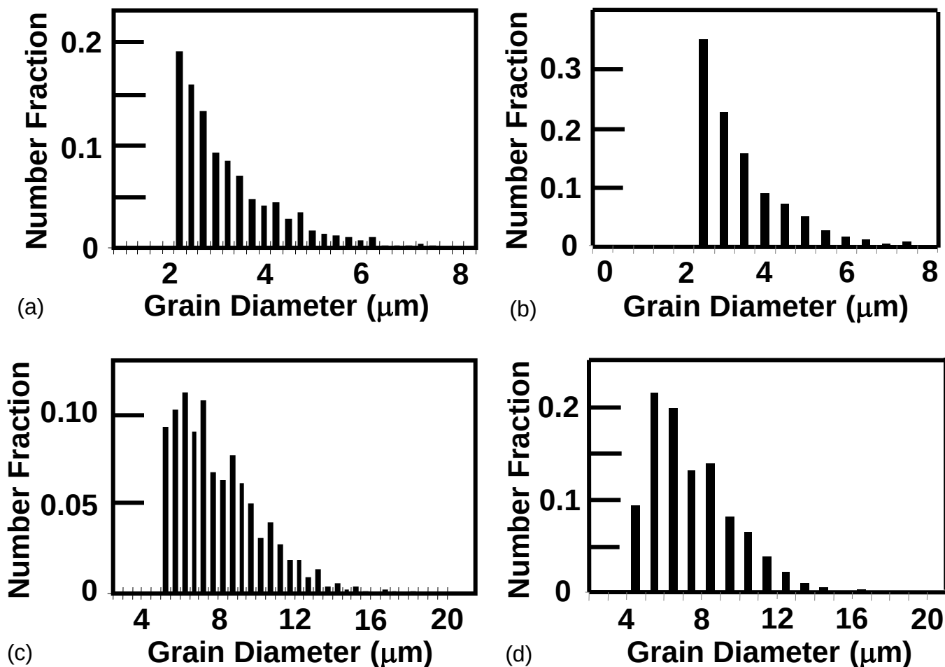
Figure 18. Approximate histograms of the gamma grain-size distribution extracted from segmented images of 230-mm-diameter LSHR extrusion OD samples which were preheated 10 minutes and compressed to a 2:1 reduction at 0.0005 \text{ s}^{-1} and a temperature of (a, b) 1339 K (1066°C) or (c, d) 1408 K (1135°C).
