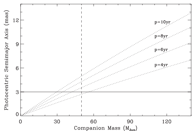
Figure 2. Companion mass sensitivity for primary mass 0.66 M_{\odot} and a 3\sigma threshold of 3 mas deviation due to circular orbital motion for GD 66. Plotted as dotted lines is the astrometric excursion as a function of companion mass for several benchmark orbital periods. The dashed line corresponds to a detectable companion mass of 50 M_{\text{Jup}} at nearly all orbital periods between 4 and 20 yr. For circular motion, the companion mass sensitivity is immune to orbital inclination, and thus the USNO astrometry rule out a wide range of low-mass, stellar and substellar companions capable of producing the O-C variations.
