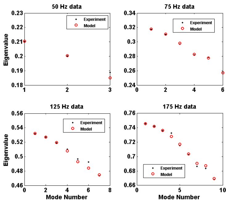
Figure 4.6.2. The figure shows the agreement between the eigenvalues estimated from data and the eigenvalues of the model in the case of Shemp.
