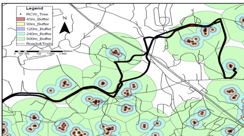
Figure 28. Training distance from RCW clusters.
