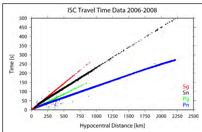
Figure 7. Travel-time distance curves for high-quality P- and S-wave phase picks, as reported by ISC from January 2006 through July 2008.
