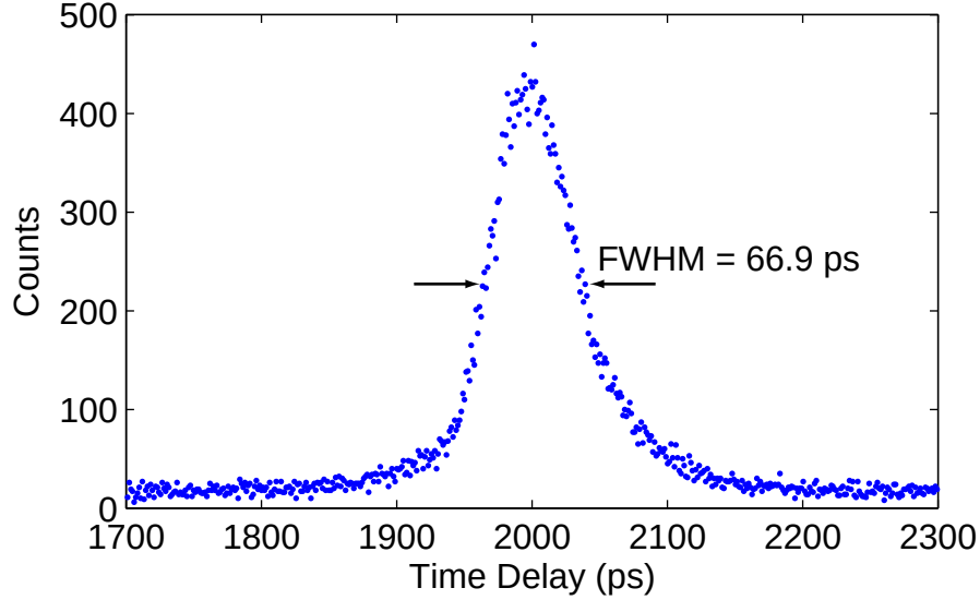
Figure 7.6: Timing histogram of 10-ps-pulsed 1.55\text{-}\mu\text{m} signal using two-step upconverter and id100 Si APD, showing system timing jitter of 66.9 ps.
