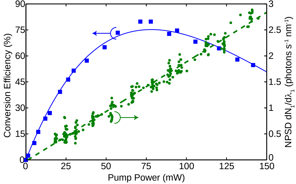
Figure 4.10: Measured DFG conversion efficiency (squares) and fit to Eq. (4.1) (solid blue), showing maximum conversion at P_{\max} = 78 mW.
