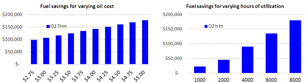
Figure 71 – Sensitivity to oil price variation of annual fuel savings (25 MMBtu/h)
