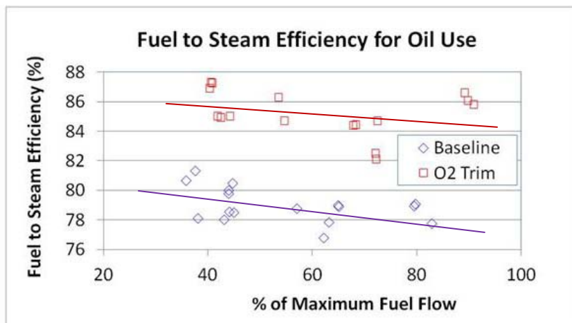
Figure 60 – Fuel to steam efficiency gains during boiler operation on No. 2 oil
