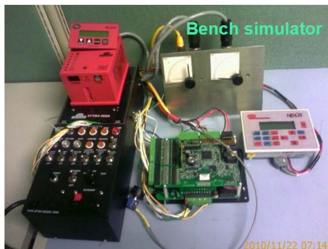
Figure 8 – The bench simulator used for open loop testing of the algorithm
