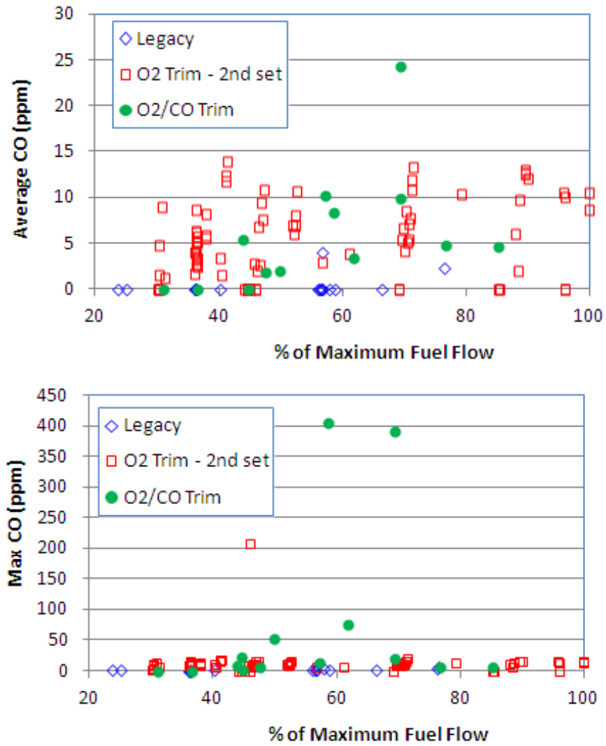
Figure 67 – CO emissions levels, average and maximum concentrations
