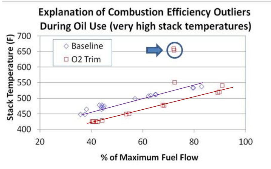
Figure 66 – Stack temperature comparisons of baseline and O 2 trim control using fuel oil
