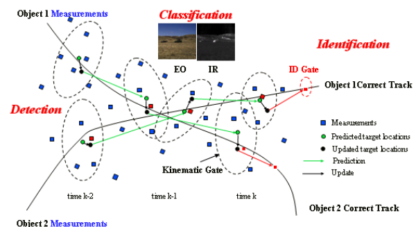
Figure 1. ID / Position Measurement Data Association.
