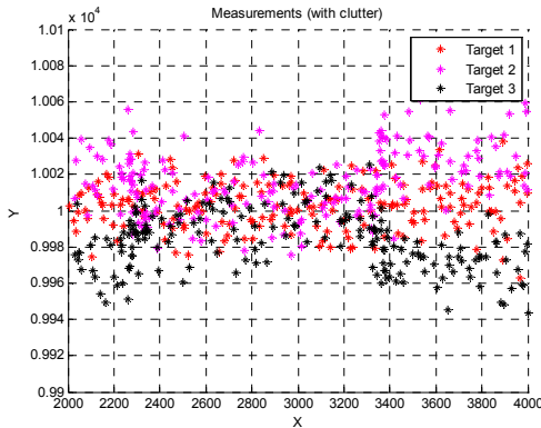
Figure 6. Track Scenario with Clutter Measurements.
