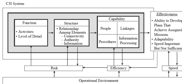
Figure 4. MOEs for C3I testing (from S. H. Starr [68]).
