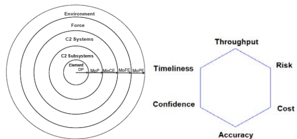
Figure 2. MOPs and MOEs relations.
