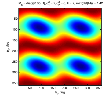
Fig. 5. Determinant of Updated FIM vs. \theta_1 and \theta_2 for Given \mathbf{M}_0 and \bar{\sigma}^2 (Example 3, k = 2 )
