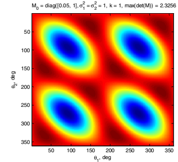
Fig. 2. Determinant of Updated FIM vs. \theta_1 and \theta_2 for Given \mathbf{M}_0 and \bar{\sigma}^2 (Example 2, k = 1 )
