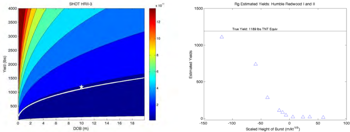
Figure 8. (Left) Moment to yield conversion using D&J and the seismic moment estimate from the R_g spectra of the 10 m DOB HUMBLE REDWOOD shot. The white line corresponds to 1.5E11 N-m. (Right) Yield estimates for all 1189-lb HR shots as a function of sHOB.
