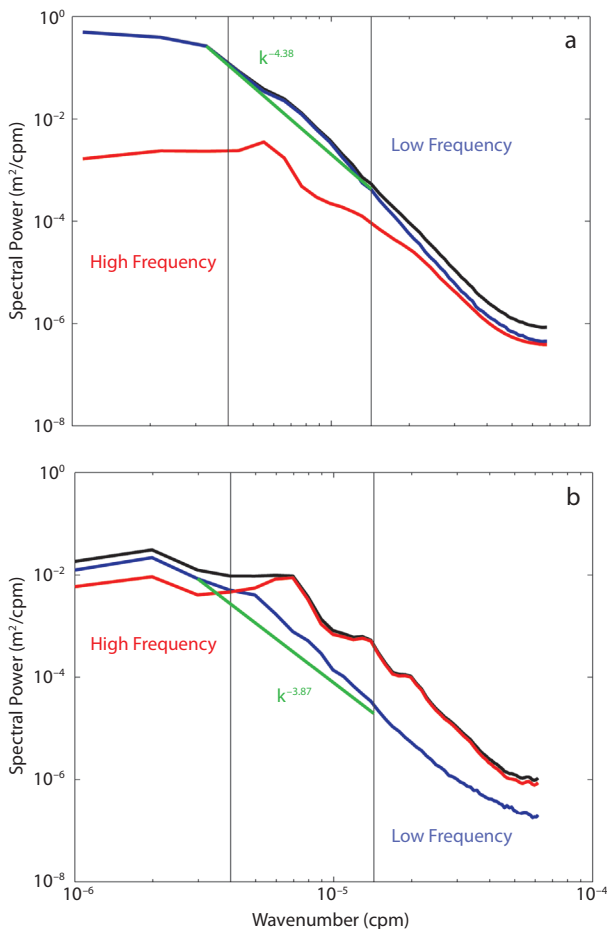
Figure 4. Wavenumber spectrum of total (black), high-frequency (red) and low-frequency (blue) sea surface height, where two days is the dividing point between low and high frequencies, for (a) Kuroshio region, a region of very strong low-frequency motions, and (b) region north of Hawai'i, in which low-frequency motions are weaker than M_2 internal tidal motions. The two regions are delineated by the westernmost and easternmost boxes, respectively, in the North Pacific in Figure 2b. Spectra are computed from a HYCOM simulation containing both tides and low-frequency atmospherically forced motions. Extra green lines are drawn in at the best-fit slopes of -4.38 and -3.87 over low-frequency motions in the same wavenumber band discussed in Xu and Fu (2011). As discussed in Le Traon et al. (2008) and Xu and Fu (2011), -11/3 and -5 slopes imply surface quasi-geostrophic and quasi-geostrophic dynamics, respectively.
