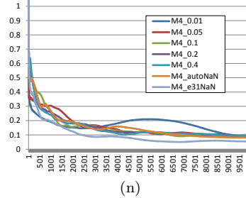
Figure 3.10: Dependence of the exploitability of the strategy given by relative frequency of use of actions in the EXP3 algorithm on the number of iterations. One row of the figures is always the game and its Nash equilibrium strategy for the row player, then follows the exploitability if the computed strategy over 10000 iterations and a detail to the first 300 iterations in the same graph.
