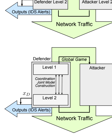
Fig. 1. Problem formulated as a global game.
