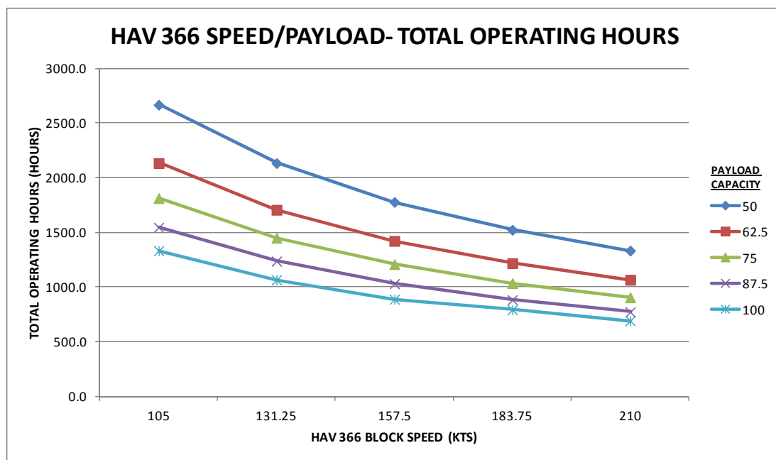
Figure 19. HAV 366 Total Operating Hours with an Increase in Payload Capacity and Block Speed of 25%, 50%, 75%, and 100%—2,500 Short Tons with a 168-Hour Mission Duration
