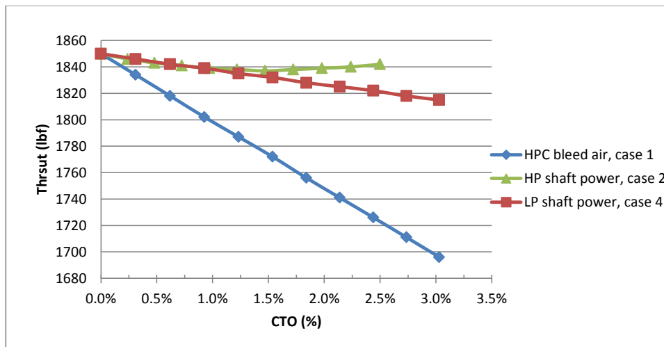
Figure IV.34. Thrust versus CTO using AEDsys: m_f = 0.35 lbm/s, Mach = 0.8, Alt = 35 kft on a standard day
