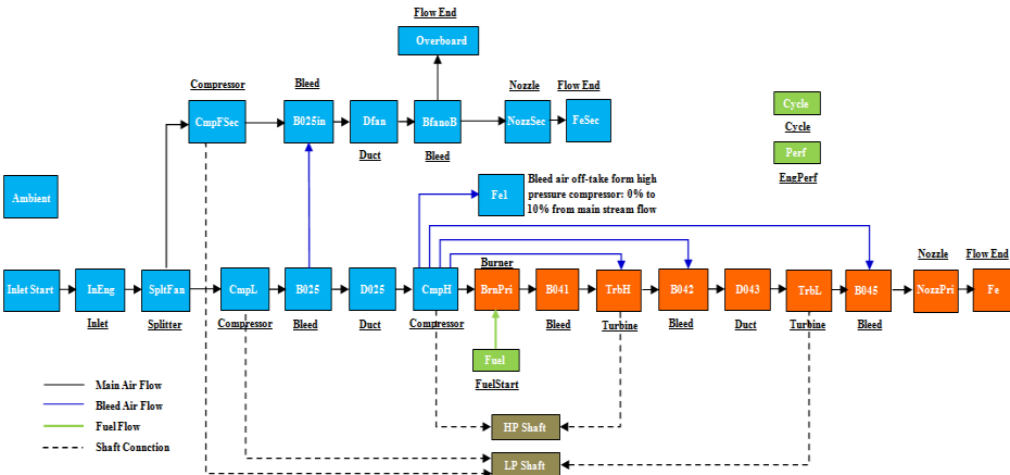
Figure III.1. High bypass turbofan baseline engine model with NPSS
