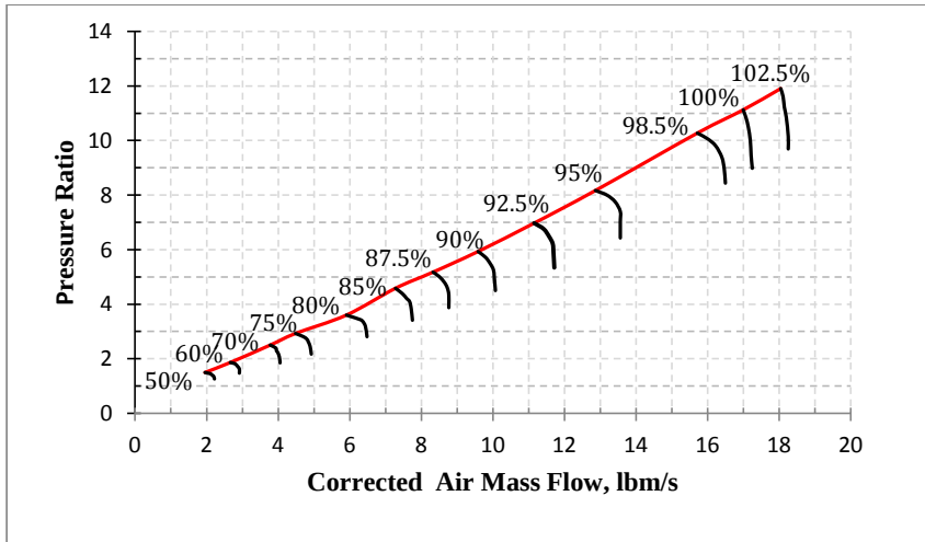
Figure III.7. Engine high pressure compressor scaled map
