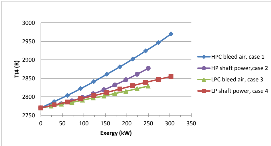
Figure C.5. Tt4 versus exergy: mf = 0.35 lbm/s, Mach = 0.8, Alt = 35 kft on standard day
