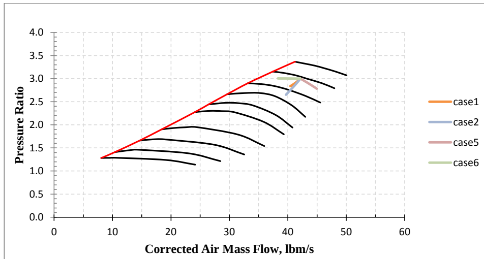
Figure C.17. LPC operating lines : w_f = 0.35 \text{ lbm/s} , \text{Mach} = 0.8 , \text{Alt} = 35 \text{ kft} on cold day
