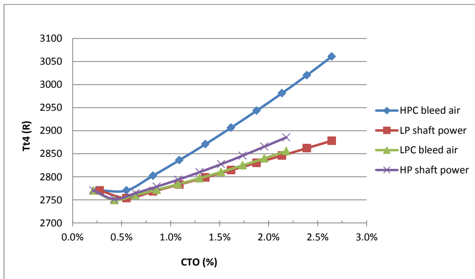
Figure IV.22. Tt4 versus CTO: Mach = 0.8, Alt = 35 kft, Fn = 1849 lbf on a standard day
