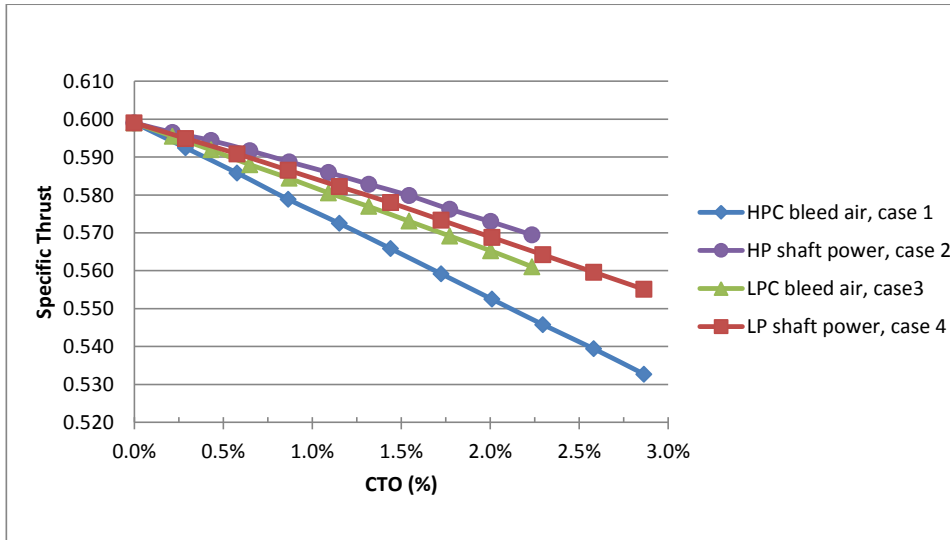
Figure IV.14. Specific thrust versus CTO: \dot{m}_f = 0.35 \text{ lbm/s} , Mach = 0.8, Alt = 35 kft on a hot day
