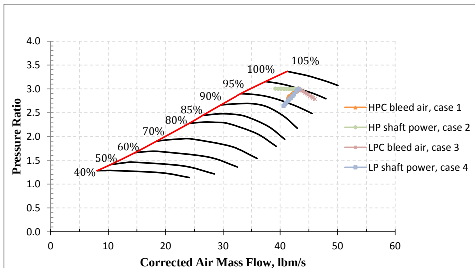
Figure IV.28. LPC operating lines: mf = 0.35 \text{ lbm/s} , Mach = 0.8 , Alt = 35 \text{ kft} on a standard day
