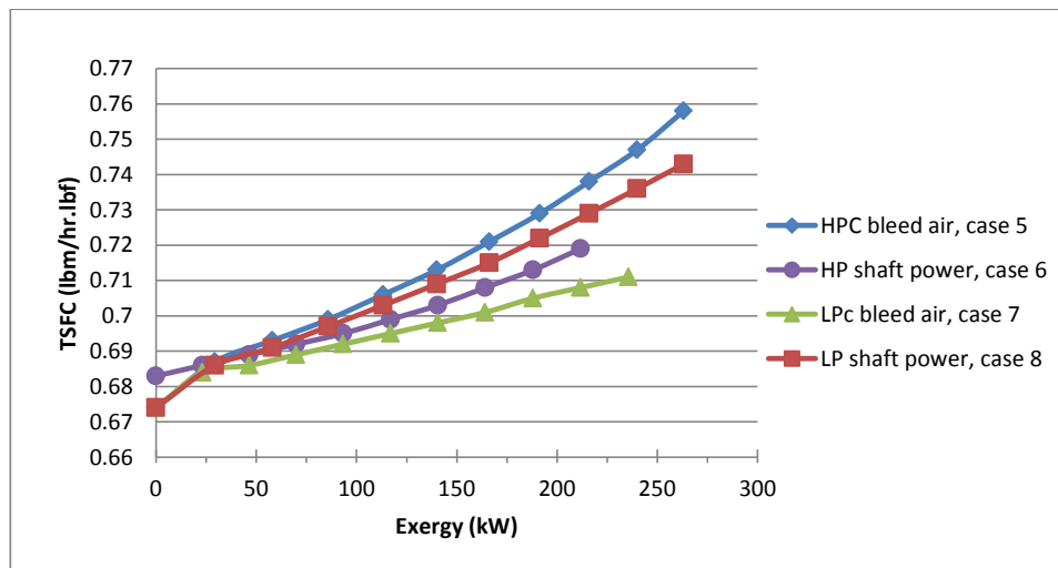
Figure C.9. TSFC versus exergy: Tt4 = 2270 R, Mach = 0.8, Alt = 35 kft on cold day
