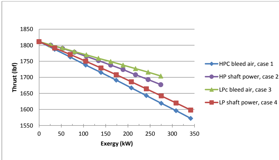
Figure C.11. Thrust versus exergy: \dot{m}_f = 0.35 \text{ lbm/s} , \text{Mach} = 0.8 , \text{Alt} = 35 \text{ kft} on hot day
