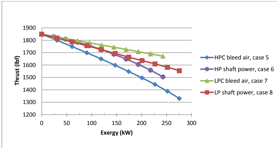
Figure C.3. Thrust versus exergy: Tt_4 = 2270 R, Mach = 0.8, Alt = 35 kft on standard day
