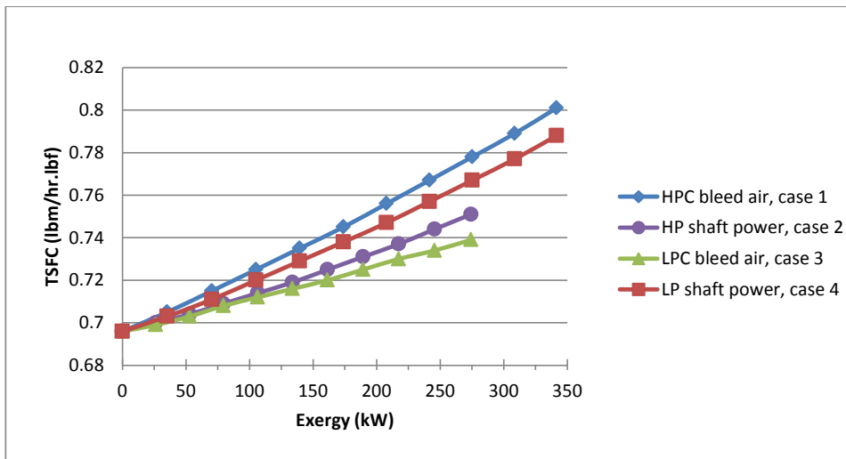
Figure C.12. TSFC versus exergy: \dot{m}_f = 0.35 \text{ lbm/s} , \text{Mach} = 0.8 , \text{Alt} = 35 \text{ kft} on hot day
