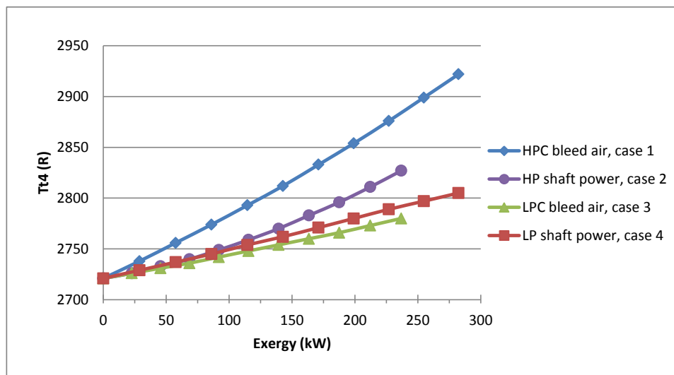
Figure C.10. Tt4 versus exergy: \dot{m}_f = 0.35 lbm/s, Mach = 0.8, Alt = 35 kft on cold day
