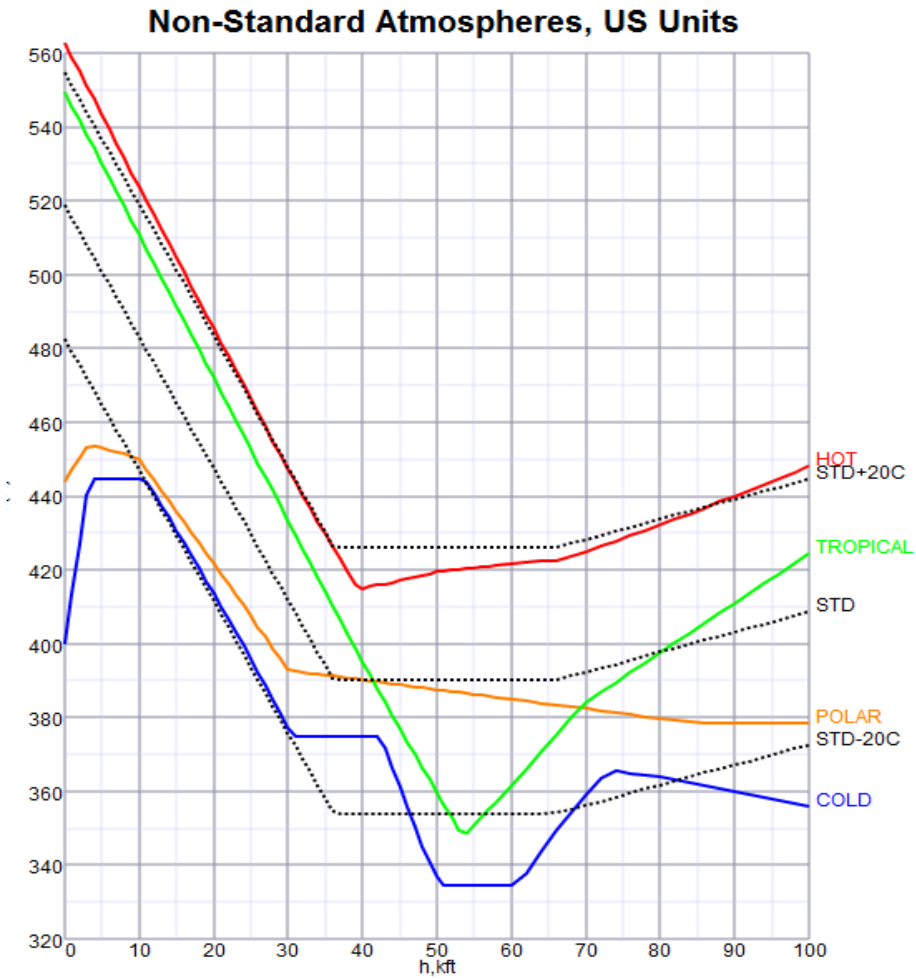
Figure B.1. MIL-STD-210A day type definition: US unit system
