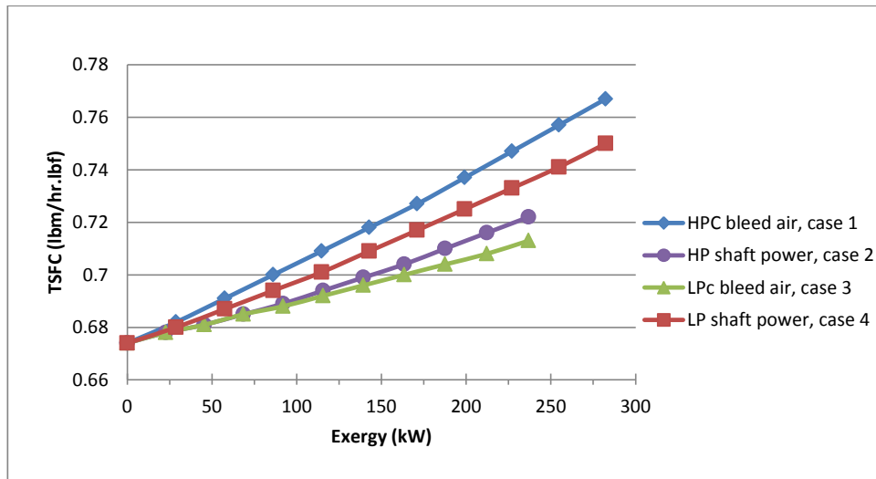
Figure C.7. TSFC versus exergy: \dot{m}_f = 0.35 lbm/s, Mach = 0.8, Alt = 35 kft on cold day
