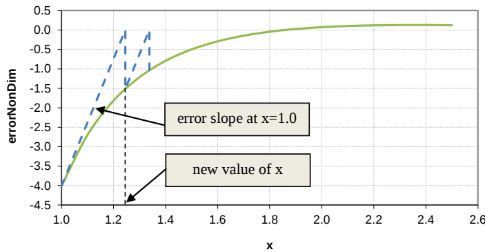
Figure II.4. NPSS Solver solution searching method
