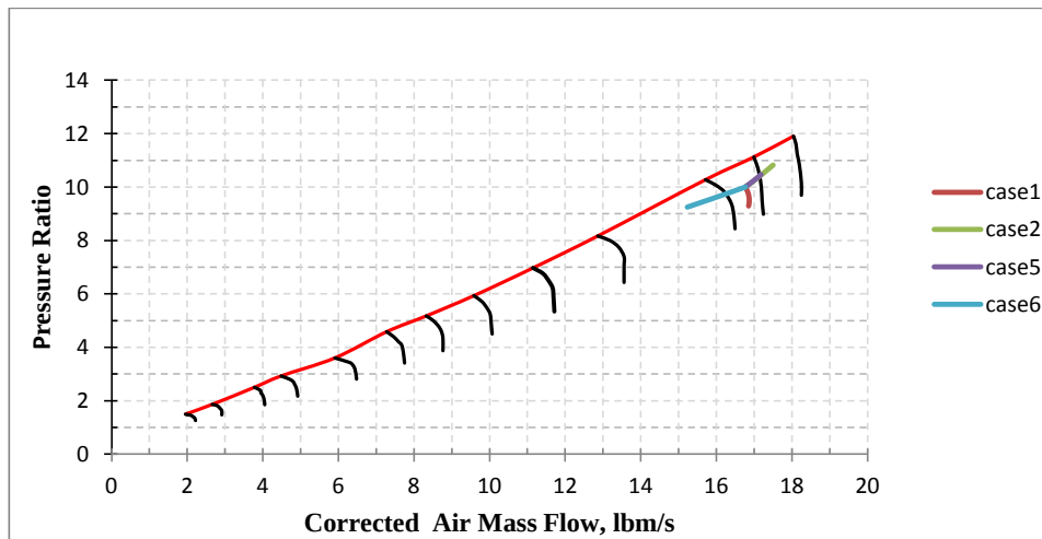
Figure C.18. HPC operating lines : w_f = 0.35 \text{ lbm/s} , \text{Mach} = 0.8 , \text{Alt} = 35 \text{ kft} on cold day
