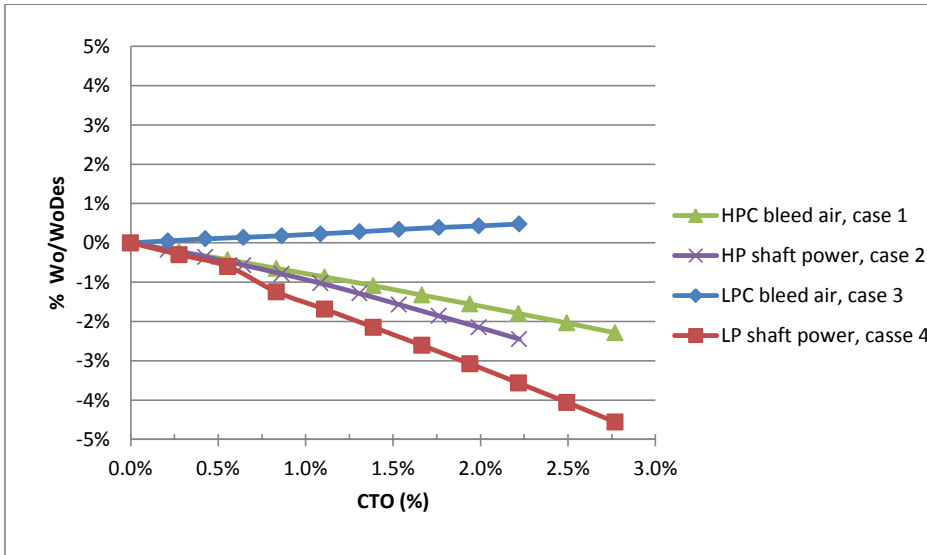
Figure IV.3 Inlet mass flow rate increment percentage versus CTO: \dot{m}_f = 0.35 \text{ lbm/s} , Mach = 0.8, Alt = 35 kft on a standard day
