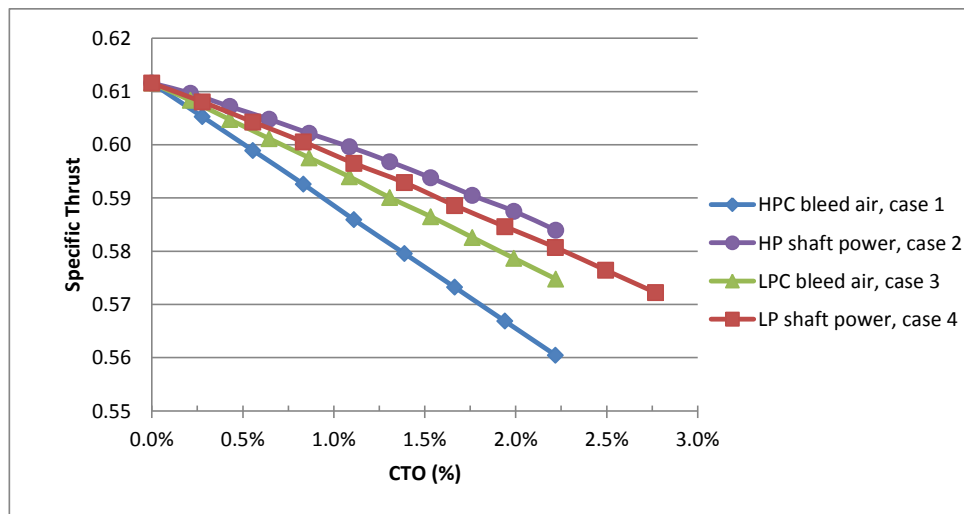
Figure IV.2. Specific thrust versus CTO: mf = 0.35 lbm/s, Mach = 0.8, Alt = 35 kft on a standard day
