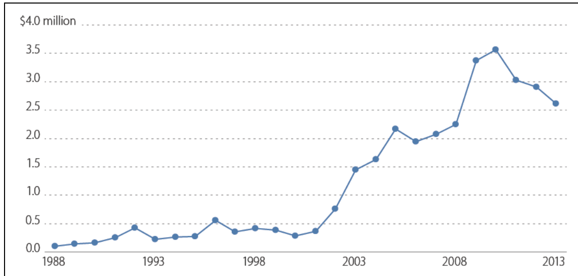
Figure 2. UAS budgets, 1988-2013
