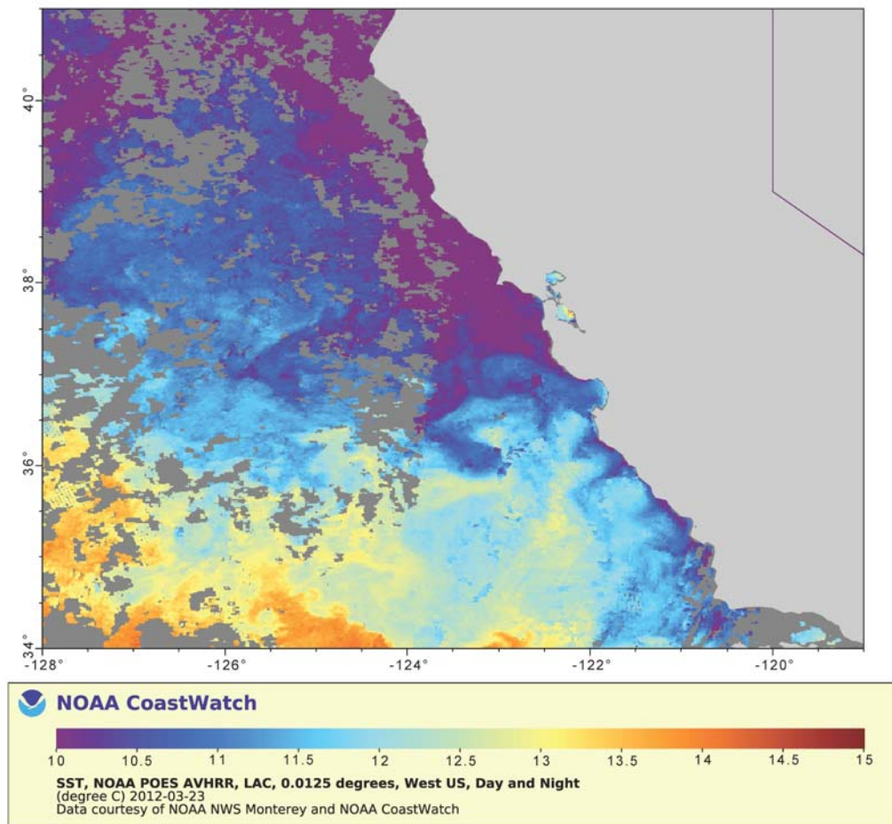
Figure 8: Advanced Very High Resolution Radiometer (AVHRR) satellite imagery of sea surface temperature ( ^{\circ} C) of the area of operation during the PaCOOS cruise of March 2012. This image was taken on 23 March 2012.
