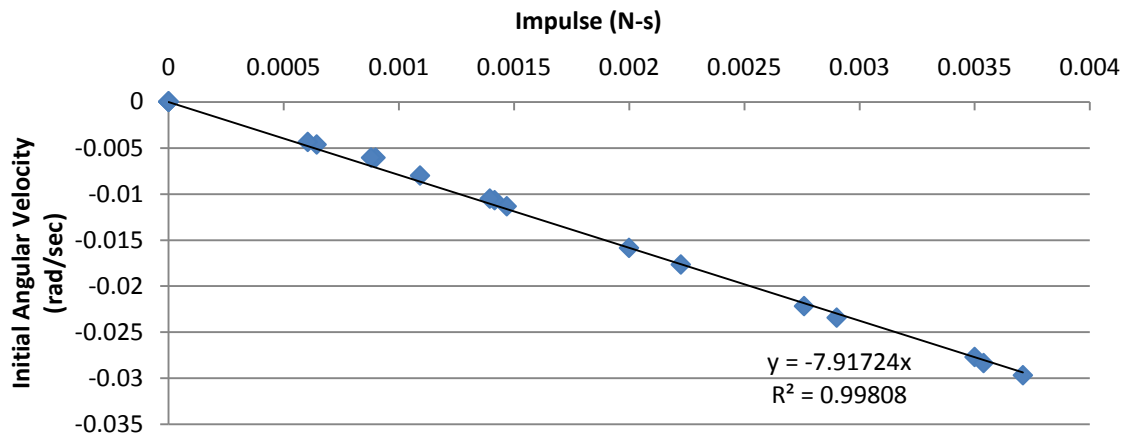
Figure 8.35. LWB Impulse vs. initial angular velocity calibration for German Bell.
