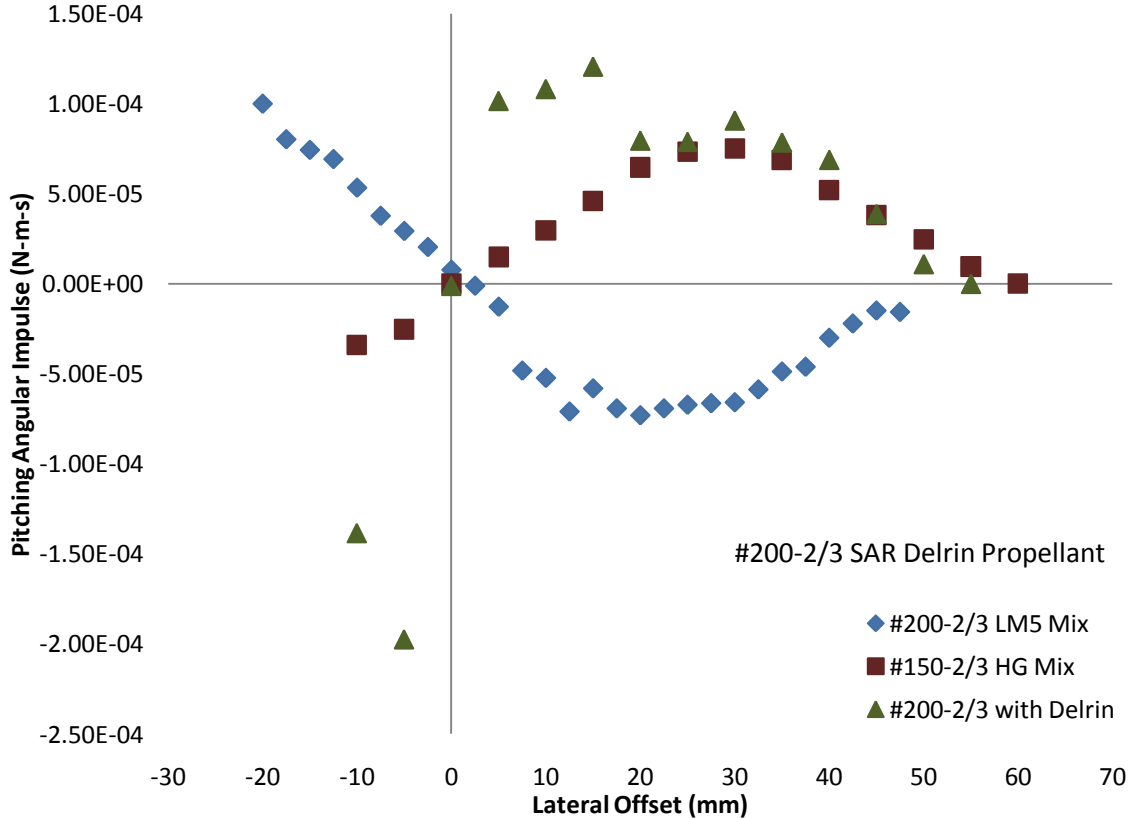
Figure 4.22. Angular pitching moments vs. lateral offset for airbreathing (AB) and “rocket mode” (RM) #200-2/3 engines.
