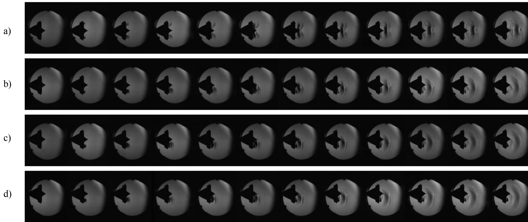
Figure 4.17. Schlieren photography of #250-2/3 with laser offset downward from engine centerline by: a) 0% D_e , b) 10% D_e , c) 20% D_e , d) 30% D_e . (~13 J pulse, ~20.5 \mu s step).
