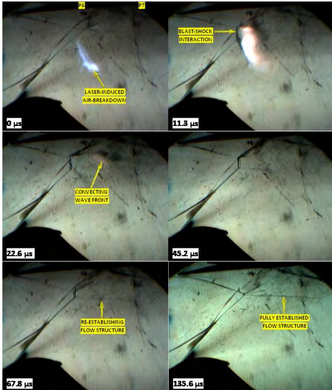
Figure 5.13: Run#16 - Laser induced blast wave interaction with oblique shocks from shroud and inlet center-body at 7.5° inclination. ( M=5.96 ; T_{\infty}=258.3 K; P_{\infty}=5.32 kPa; E_p=187\pm 19 J)
