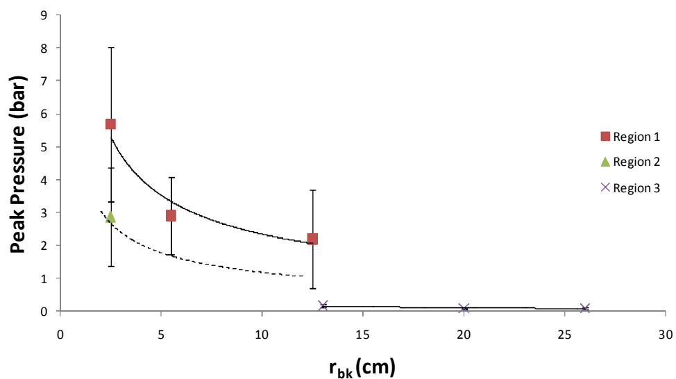
Figure 1.14: Run #7—Peak surface pressure vs. distance from laser focal line. ( P_{\infty} = 150 mbar; E_p = 222 ± 23 J)
