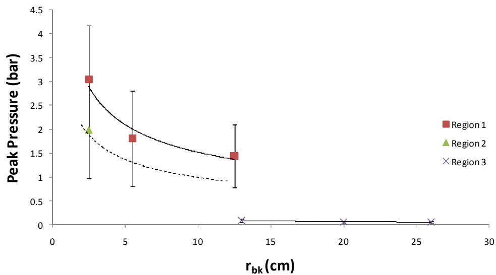
Figure 1.13: Run #1—Peak surface pressure vs. distance from laser line focus. ( P_{\infty} = 60 mbar; E_p = 172 ± 17 J)
