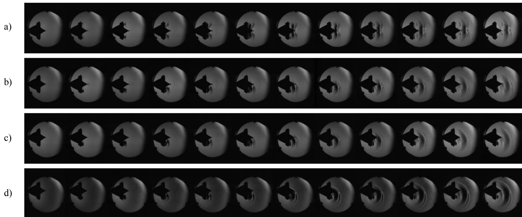
Figure 4.16. Schlieren photography of #200-2/3 with laser offset downward from engine centerline by: a) 0% D_e , b) 10% D_e , c) 20% D_e , d) 30% D_e . (~13 J pulse, ~20.5 \mu\text{s} step).
