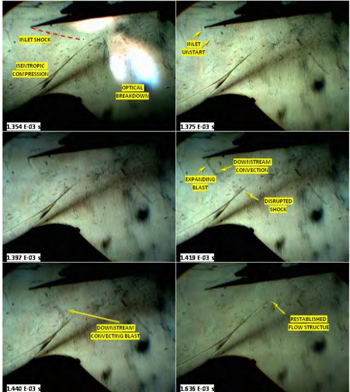
Figure 5.23: Run#21 - Laser induced blast wave interaction with oblique inlet shocks and shroud under-surface. Model and shroud at -7.5^\circ inclination. ( M=9.44 , T_\infty = 108 K, P_\infty = 0.301 kPa, E_p=196\pm20 J)
