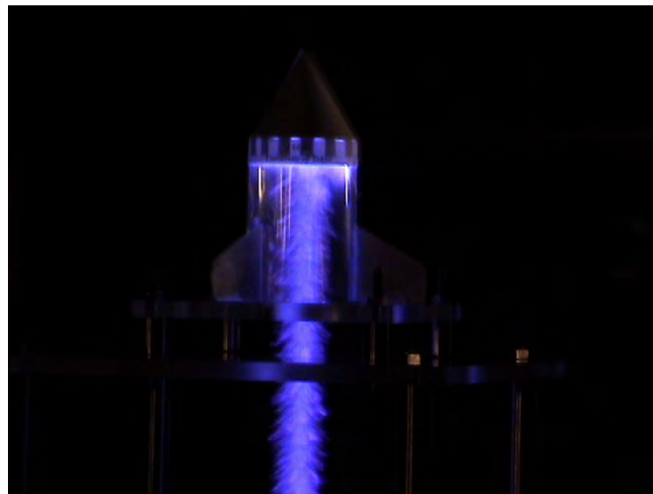
Figure 1.5 Microwave-powered Lightcraft (Nakagawa et al., 2003)
