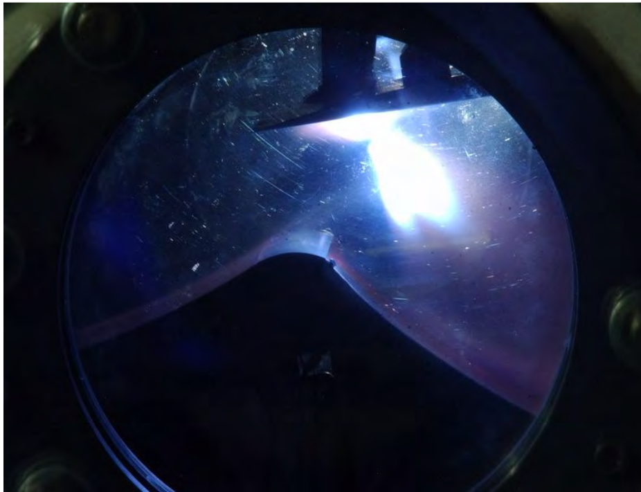
Figure 5.24: Run#21 - Long exposure photograph of bifurcated air-breakdown geometry across inlet gap, and secondary breakdown on shroud undersurface.
