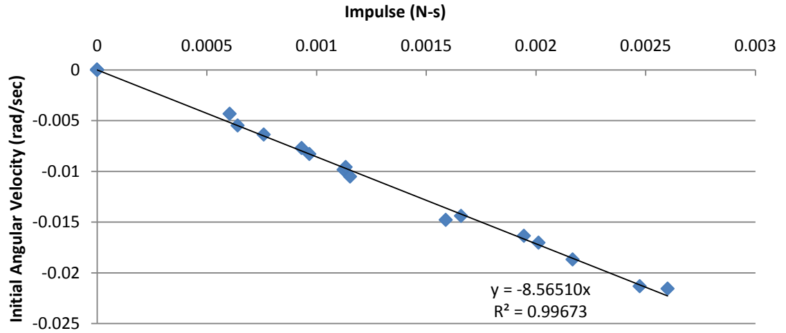
Figure 8.34. LWB Impulse vs. initial angular velocity calibration for #250-2/3.
