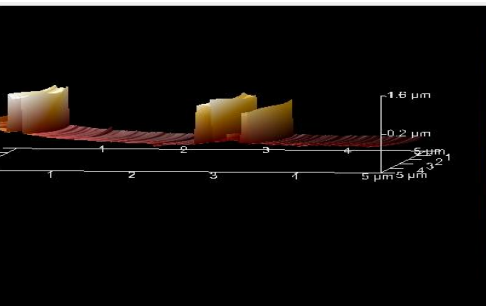
Figure 14: AFM of BaTiO 3 thin film, substrate Temperature=100°C.
