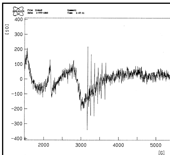
Figure 6 : EPR spectrum for Mn: BaFeO 3 thin film
