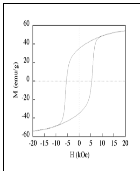
Figure 4: Hysteresis loop for sample 1 at room temperature.
