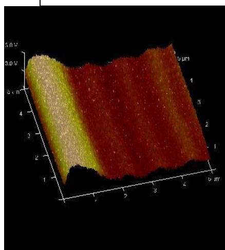
Figure 14: BaTiO3:Mn P(O 5mTorr), T=400C
