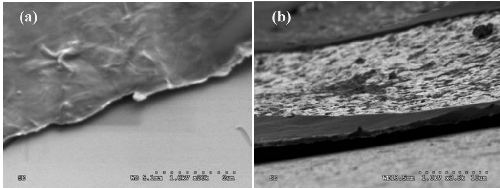
Figure 9 (a) graphene paper entirely coated with PMMA on both sides and (b) graphene/PMMA paper with PMMA partially peeled off.
