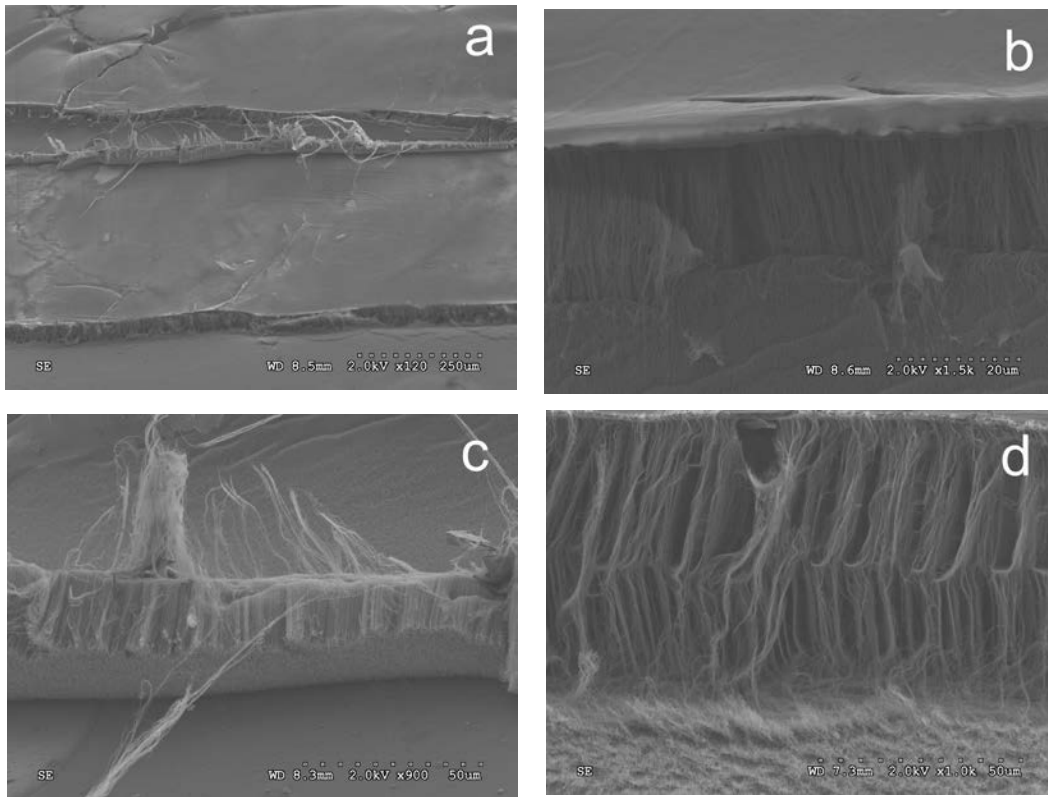
Figure 15 SEM of the transferred three-layered VA-CNT/graphene. (a) the over view of the three layered structure; (b), (c) and (d) are the details of the first, second and third layer, respectively.
