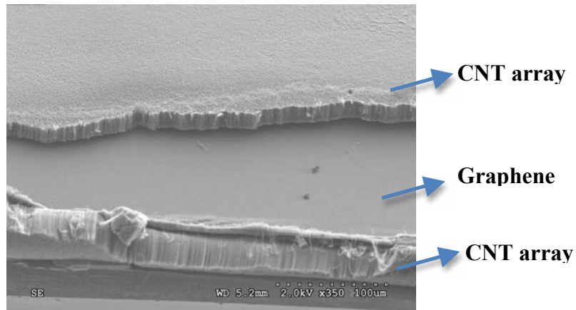
Figure 13 SEM of the assembled two-layered VA-CNT/graphene
