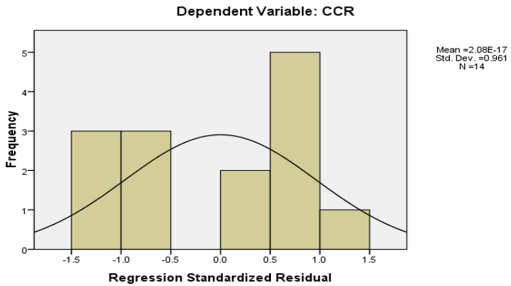
Figure 7: Forward/Mixed Stepwise Regression Histogram
