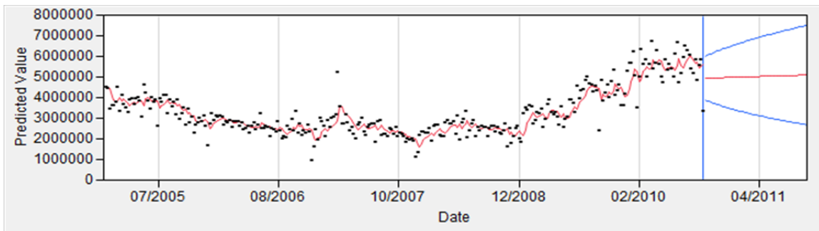
ARIMA(0,1,1) Method, Weekly Afghanistan+ Demand
