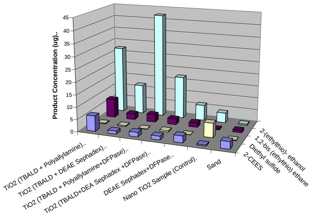
Figure 7. Residual 2-CEES and reaction products after 24-h contamination of half-mustard vapor on templated titania samples compared to commercially obtained nanoTiO 2 control sample (NanoActive TiO 2 ).
