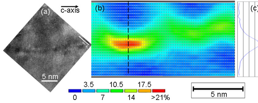
Fig. 9 Two-beam TEM image (a) and the corresponding SSA image (b) of a section of a sidewall QW near the bottom of the QW NR. Part (c) shows the line-scan indium content profile along the vertical dashed line in part (b).
