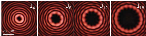
Fig. 3. Selected higher-order Bessel beams at low intensity. The ring intensity features of the beams are modulated due to the 2\pi - modulo phase mask.
