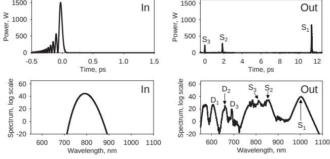
FIG. 2: Top row: Input and output temporal waveforms for the case of the propagation of an Airy pulse with -60,000 \text{ fs}^3 cubic spectral phase in a 1 m-long nonlinear fiber with the parameters described in the text. Bottom row: Corresponding spectra. Solitons and dispersive waves are marked with letters S_i and D_i , where the subscript indicates the order of appearance of these features.
