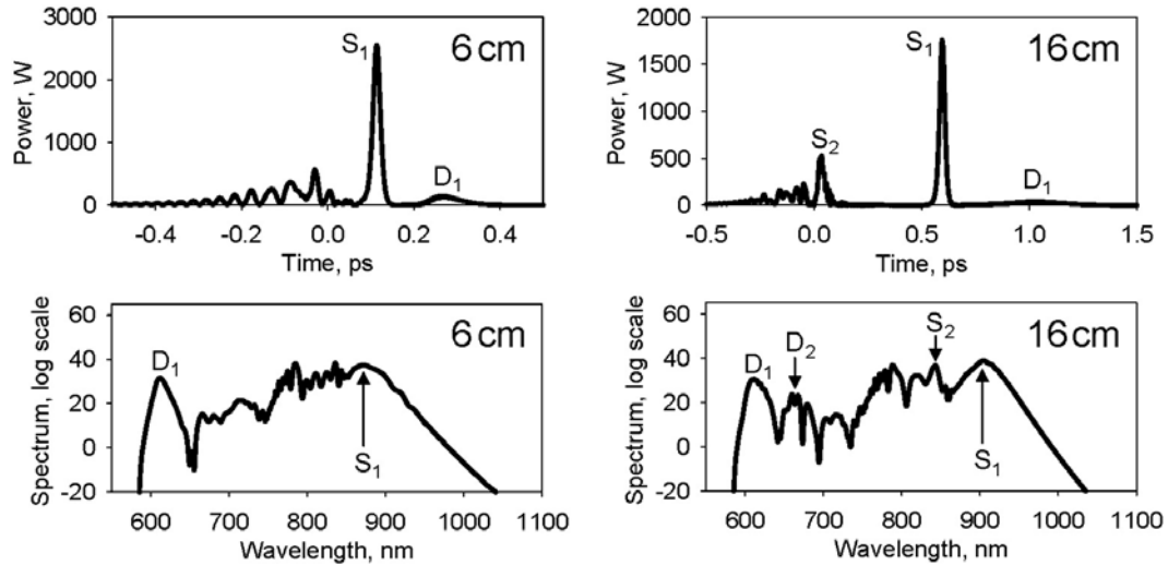
Figure 3: Top row, left: Temporal waveforms of the Airy pulse with -60,000 \text{ fs}^3 cubic spectral phase after 6 cm propagation in the fiber. The main peak of the Airy waveform has produced a soliton-dispersive wave pair and is nearly regenerated. Right: Same after 16 cm propagation. The regenerated main pair peak of the pulse has produced another soliton-dispersive wave pair. Bottom row: Corresponding spectra.
