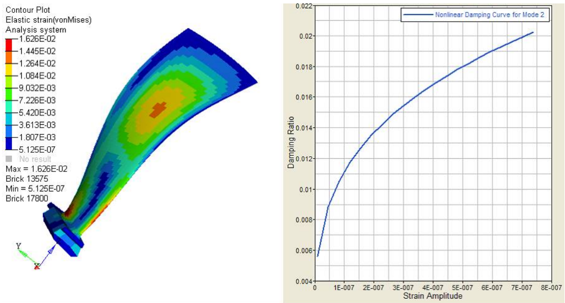
FIGURE 20 Second Mode Damping
