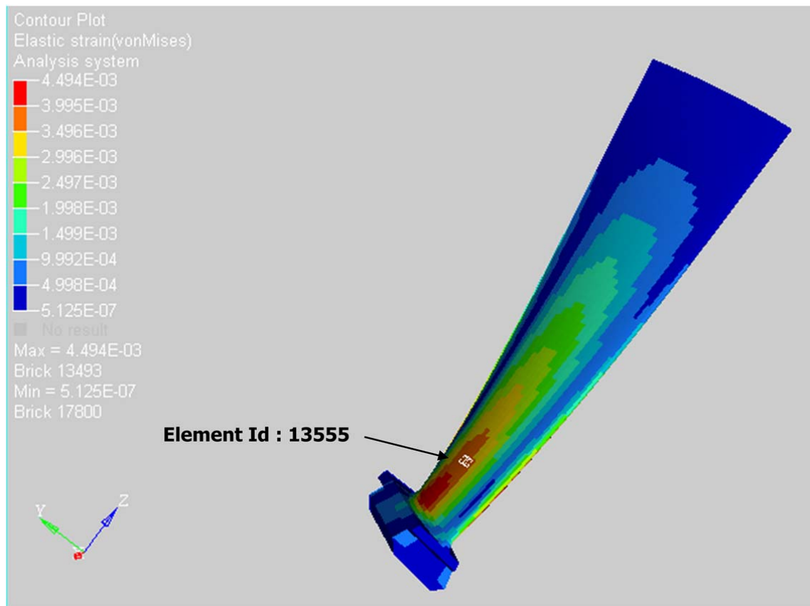
FIGURE 18 Reference Element
