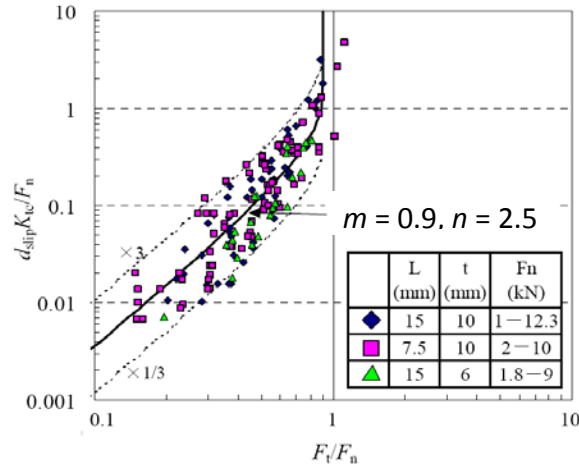
FIGURE 15 Asai et al Experimental Result for Micro-Slip
