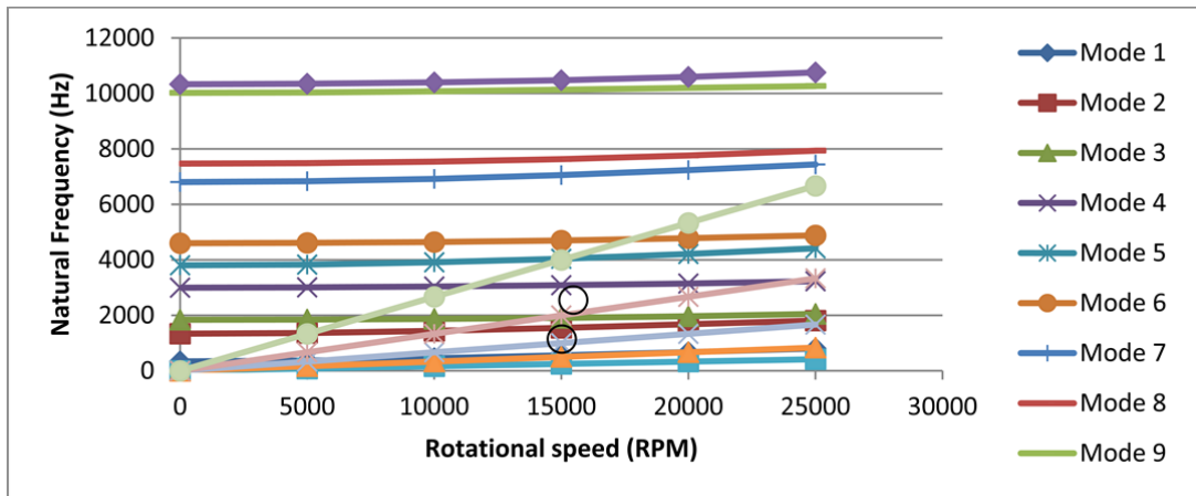
FIGURE 17 Campbell diagram of first stage of SO-3 engine rotor blade
