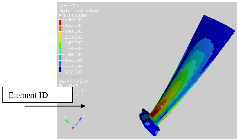
Fig. 8 Reference Element
