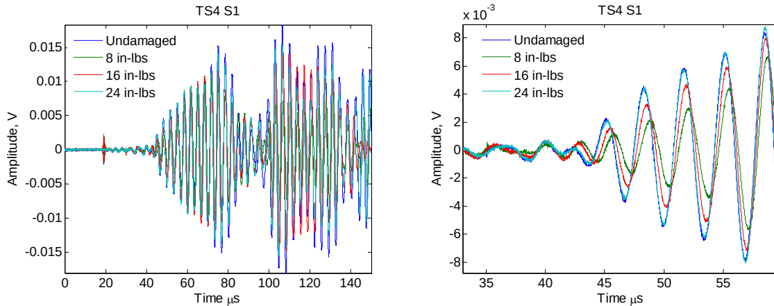
Figure 64 Elastic wave signals collected for the PNP satellite bolted joint subjected to different torque levels.
