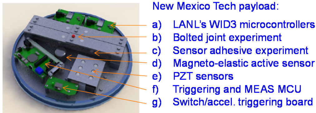
Figure 80 Schematics of New Mexico Tech payload.
