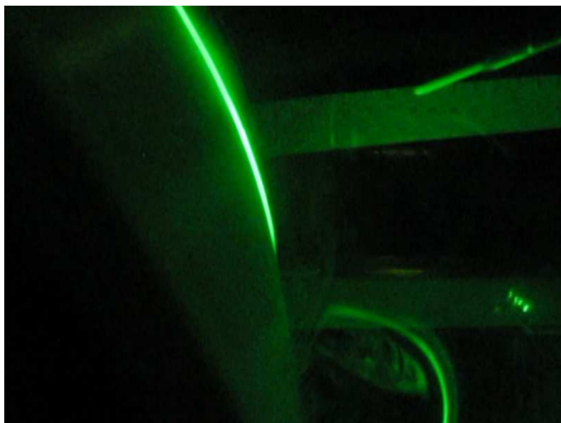
Figure 27 Flow structure of within the free stream rising incense being swept along with the boundary layer over the reversely (clockwise) rotated drum
