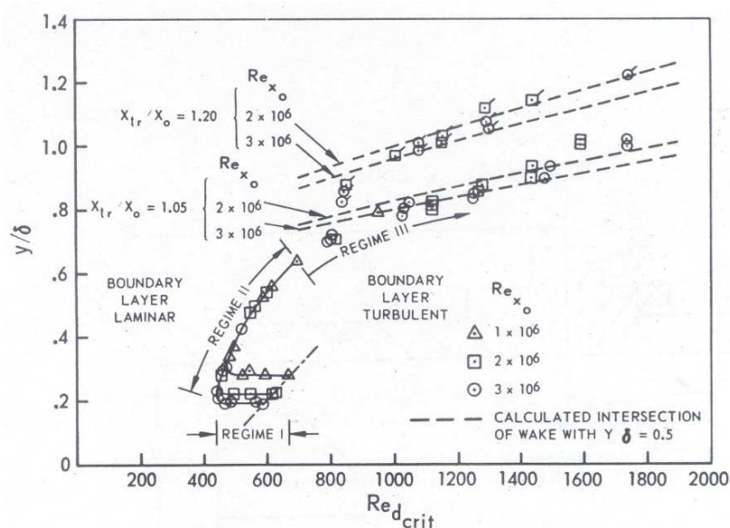
Figure 4 Variation of the critical Reynolds number with the ratio of transverse distance of the top of the sphere from the pipe wall, y , to boundary layer thickness, \delta , reproduced from Hall [10]
