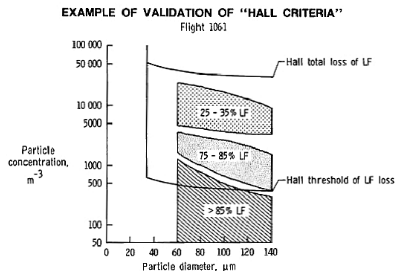
Figure 2 Comparison of results from the NASA LEFT program to the „Hall Criteria“, reproduced from Davis et al. [6]
