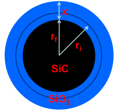
Fig. 1. Diagram showing initial ( r_i ) and final ( r_f ) SiC thickness after oxidation and \text{SiO}_2 thickness x .
