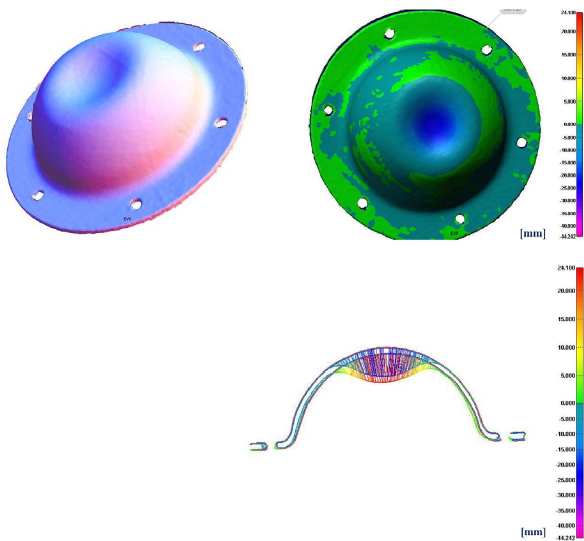
Figure B23. Nose: Full surface scan, contour map and cross-section
