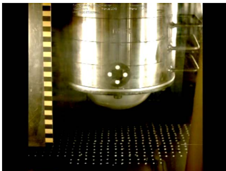
Figure 9. Frame from a high speed video showing the carriage falling towards the plate prior to impact. Tiger tape on the left hand side of the frame and tracking markers attached to the lowest ballast tablet are for video motion analysis.
