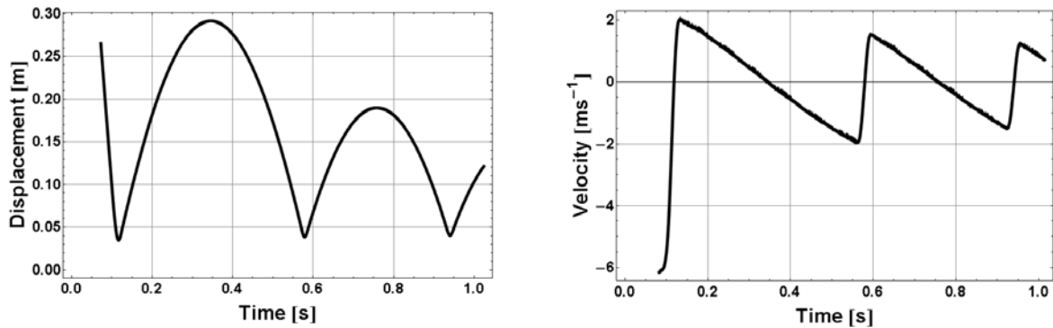
Figure B16. Displacement and velocity of the falling carriage
