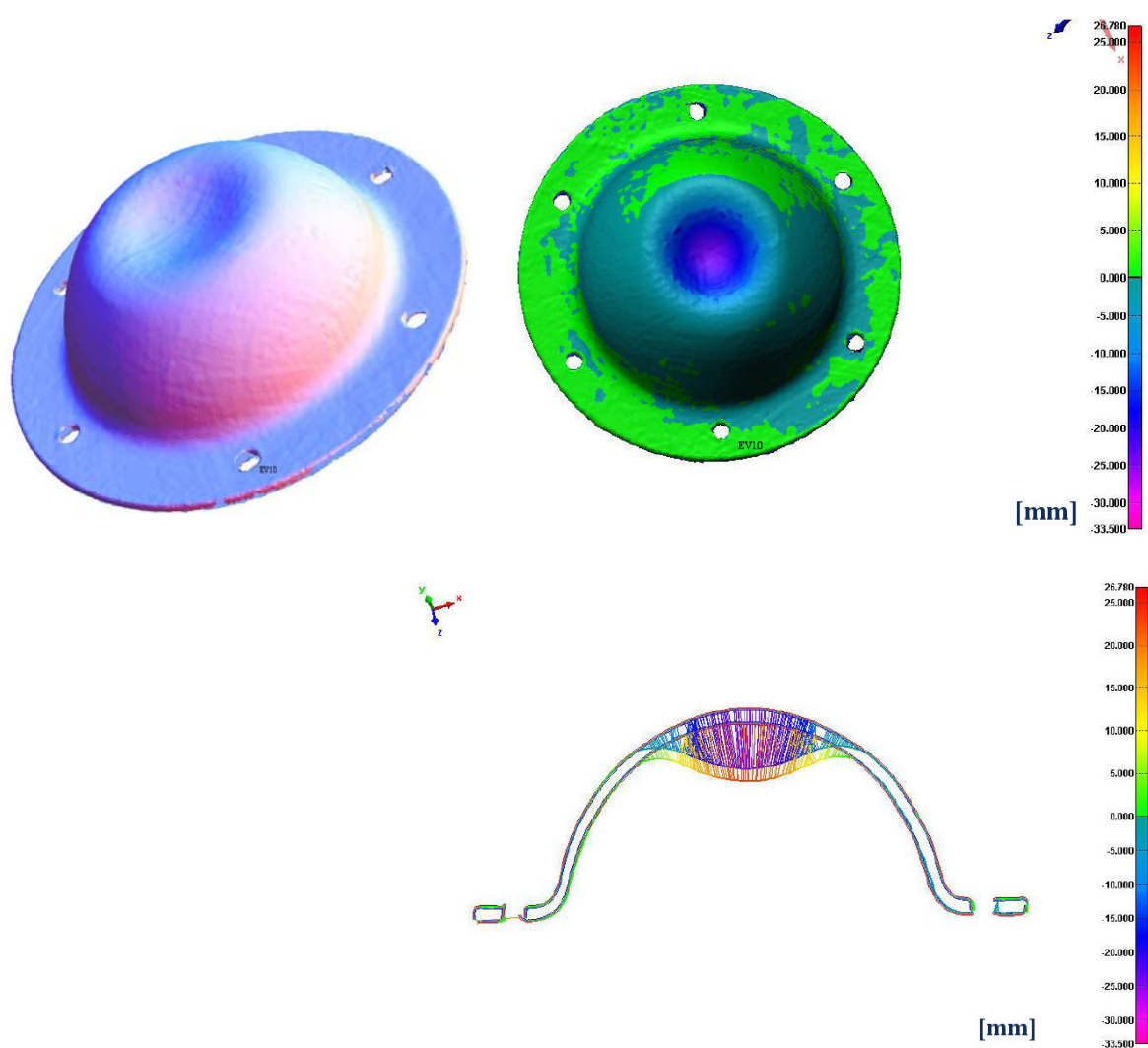
Figure B26. Nose: 3D Full surface scan, contour map and cross-section
