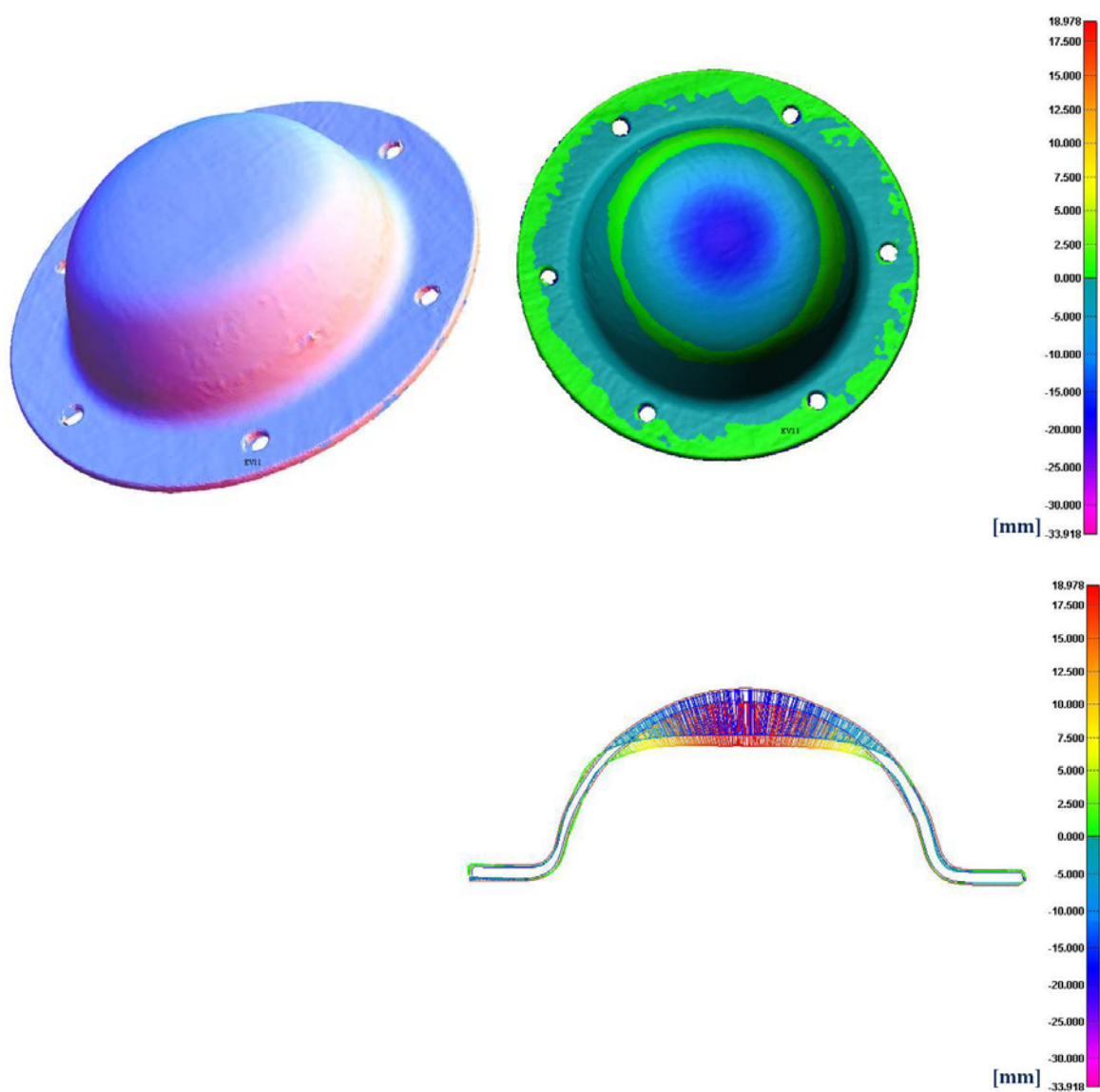
Figure B15. Nose: Full surface scan, contour map and cross-section
