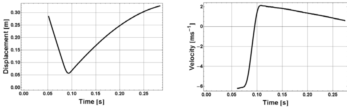
Figure B4. Displacement and velocity of the falling carriage
