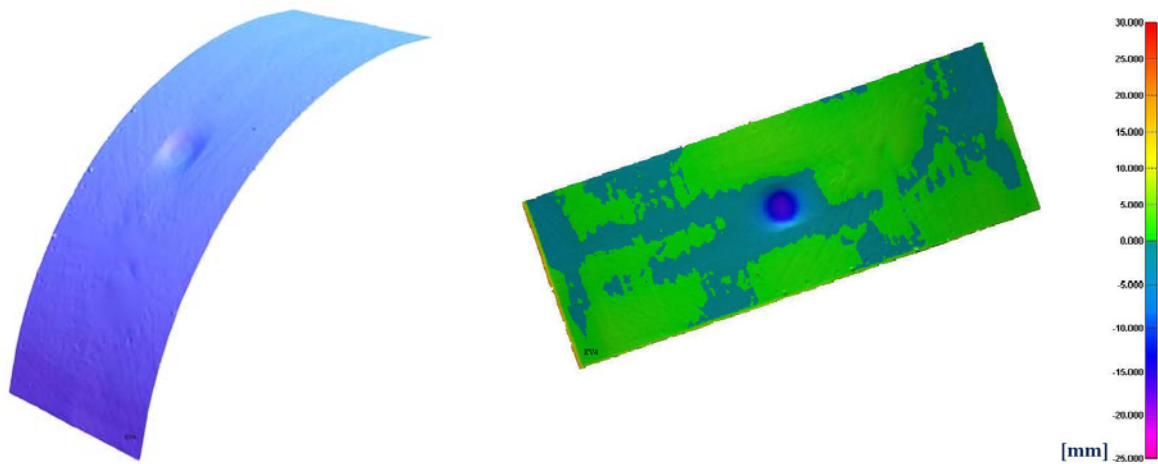
Figure B8. Dented Plate: Surface scan &amp; contour map
