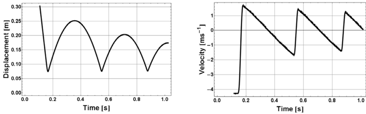
Figure B10. Displacement and velocity of the falling carriage
