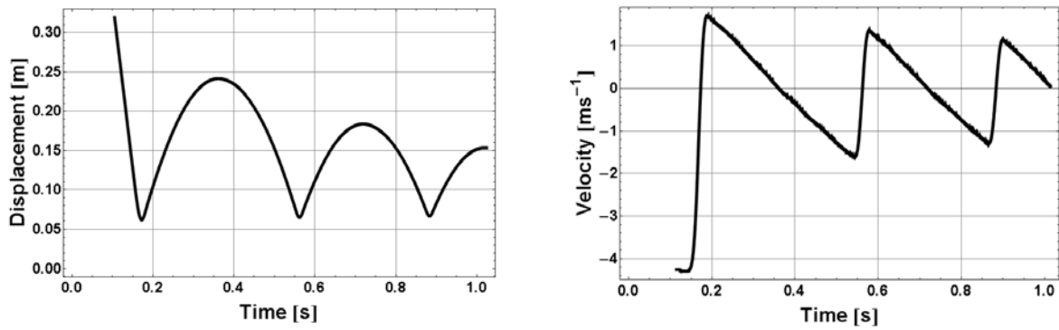
Figure B19. Displacement and velocity of the falling carriage
