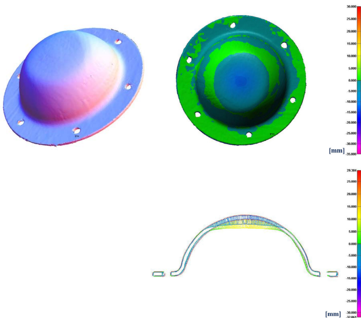
Figure B9. Nose: Full surface scan, contour map and cross-section
