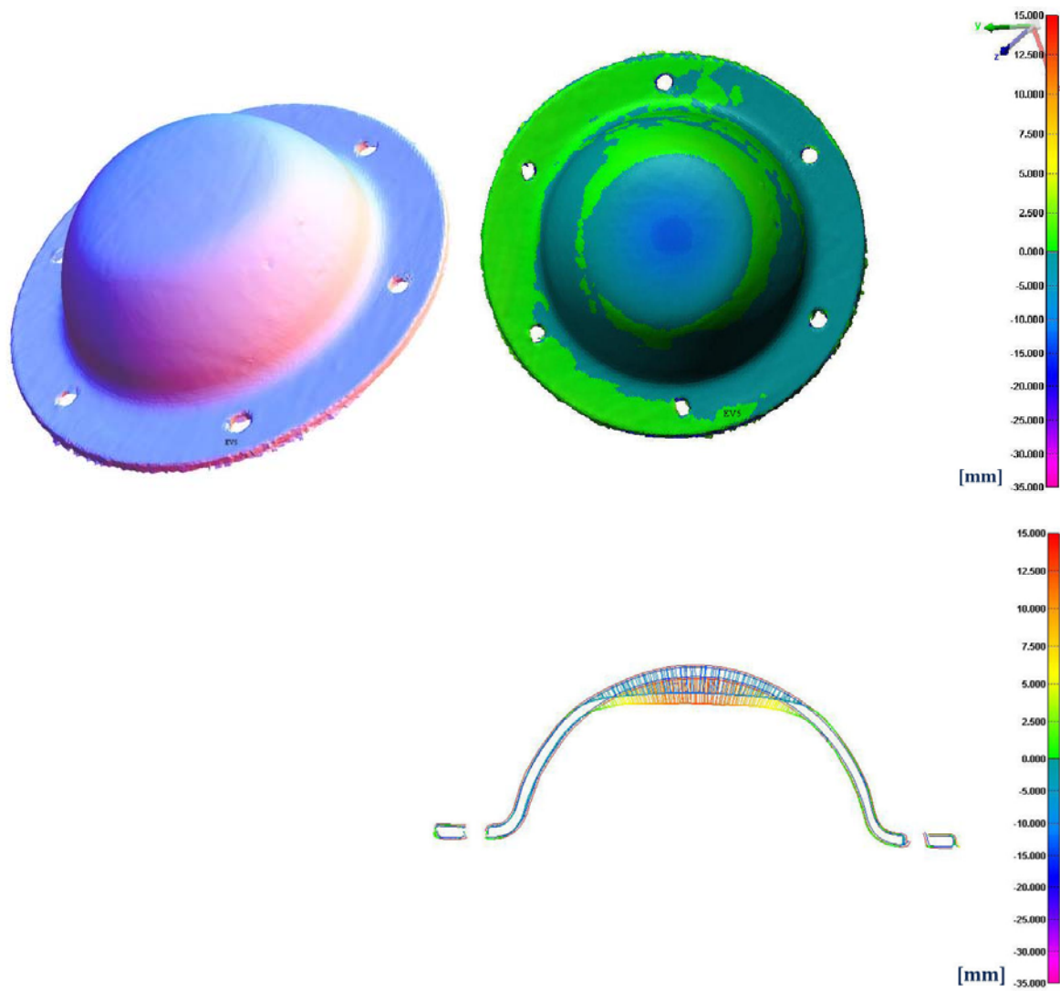
Figure B12. Nose: Full surface scan, contour map and cross-section
