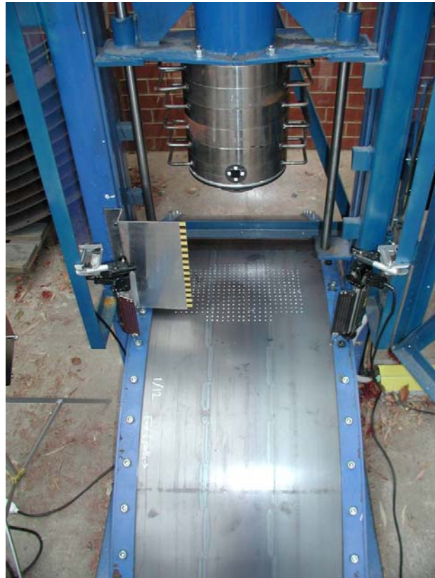
Figure 2. Drop tower showing ballast tablets attached to the drop carriage above the clamped model hull plate prior to a drop. The reference marks on the lowest ballast tablet and the tiger tape attached to the left hand side tower upright are for video motion analysis.
