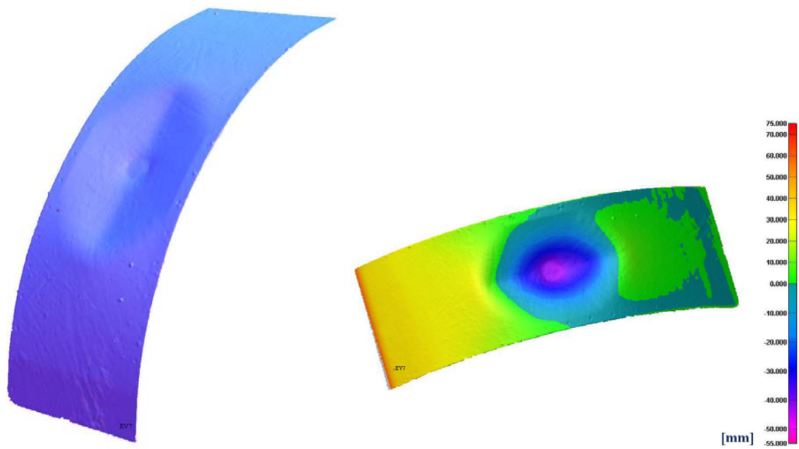
Figure B17. Dented Plate: Surface scan & contour map
