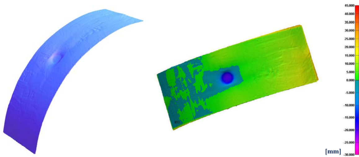
Figure B2. Dented Plate: Surface scan & contour map
