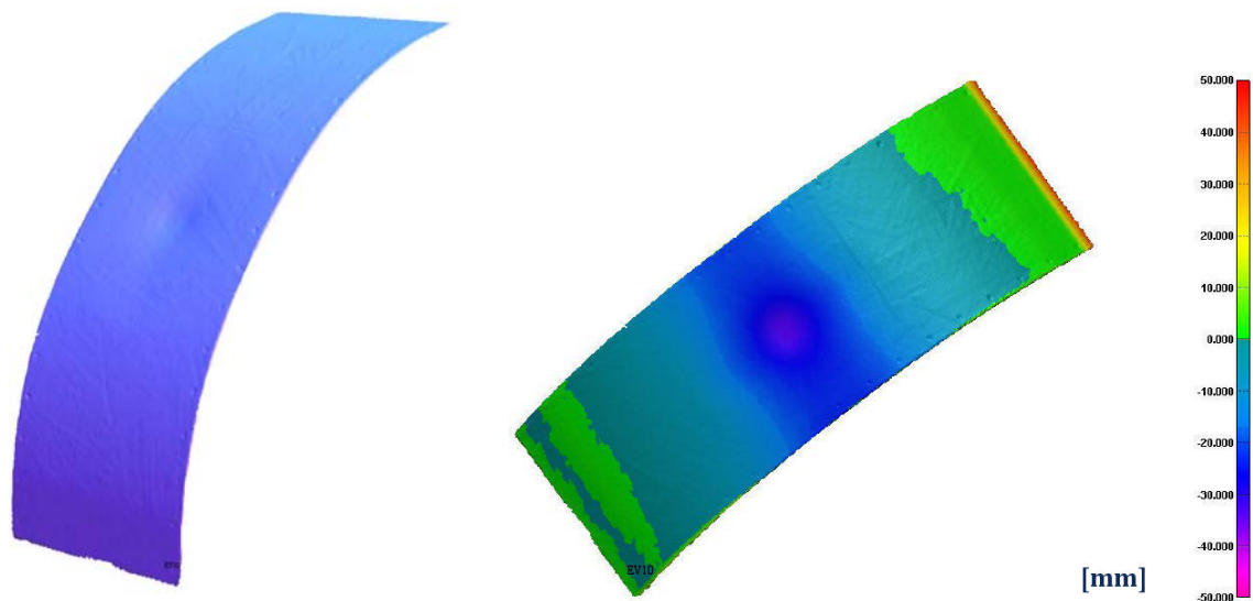
Figure B25. Dented Plate: Surface scan &amp; contour map
