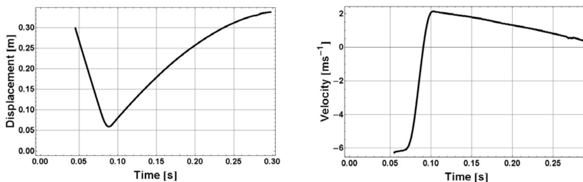
Figure B1. Displacement and velocity of the falling carriage
