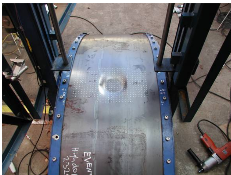
Figure 8. Steel plate with T-stiffeners clamped to the drop tower form, post impact
