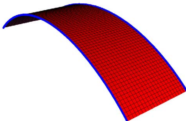
Figure 7. Plate showing boundary conditions as it is fixed in the drop tower. Blue edges clamped, otherwise free.
