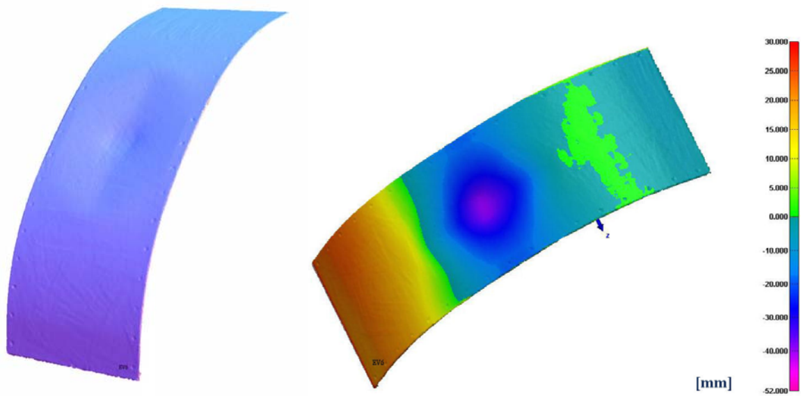
Figure B27. Dented Plate: Surface scan &amp; contour map
