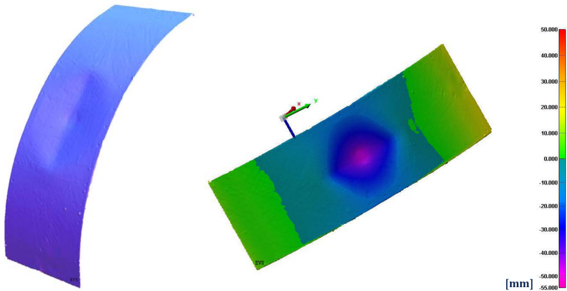
Figure B20. Dented Plate: Surface scan &amp; contour map
