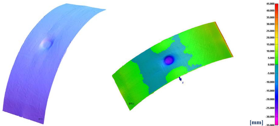
Figure B14. Dented Plate: Surface scan &amp; contour map
