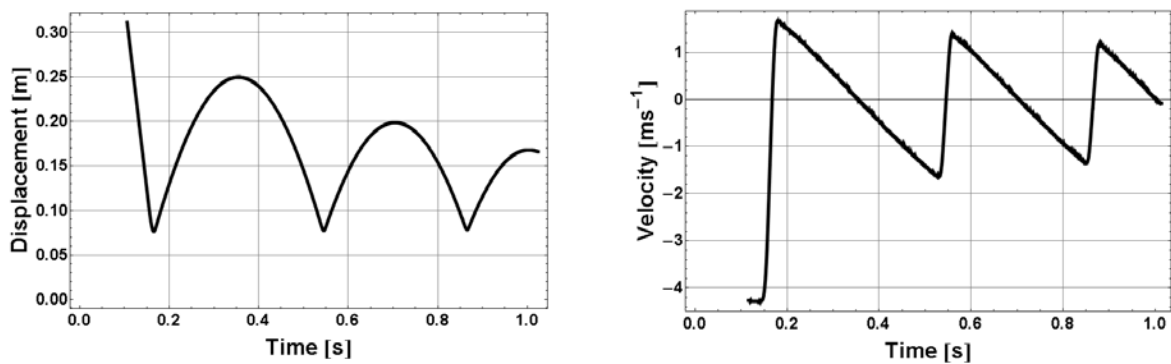
Figure B7. Displacement and velocity of the falling carriage
