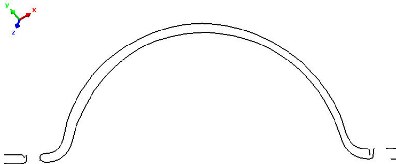
Figure 4. Cross section taken from a 3D scan of a nose showing a degree of thinning caused by the manufacturing process
