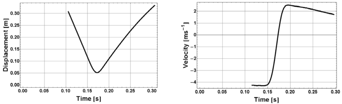
Figure B24. Carriage fall
