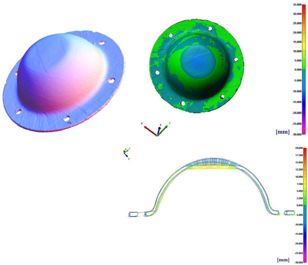
Figure B21. Nose: Full surface scan, contour map and cross-section
