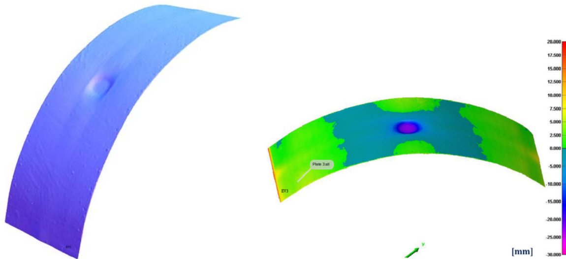
Figure B5. Dented Plate: Surface scan &amp; contour map
