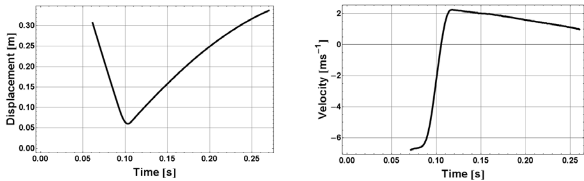
Figure B13. Displacement and velocity of the falling carriage
