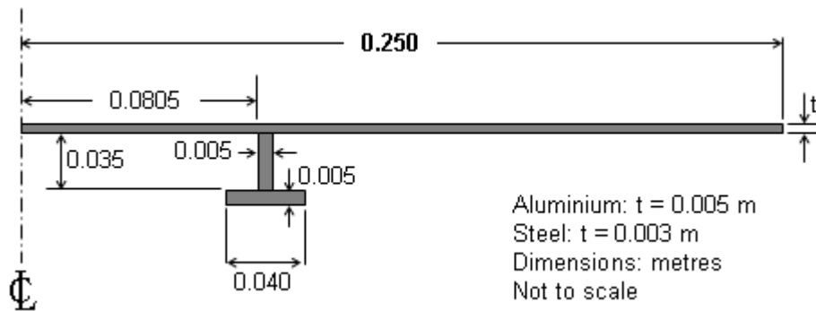
Figure 5. Section of stiffened model hull plate. (Unstiffened plate has equal shared dimensions. Width dimension does not include the plate material held by clamping along the plate's long edges).
