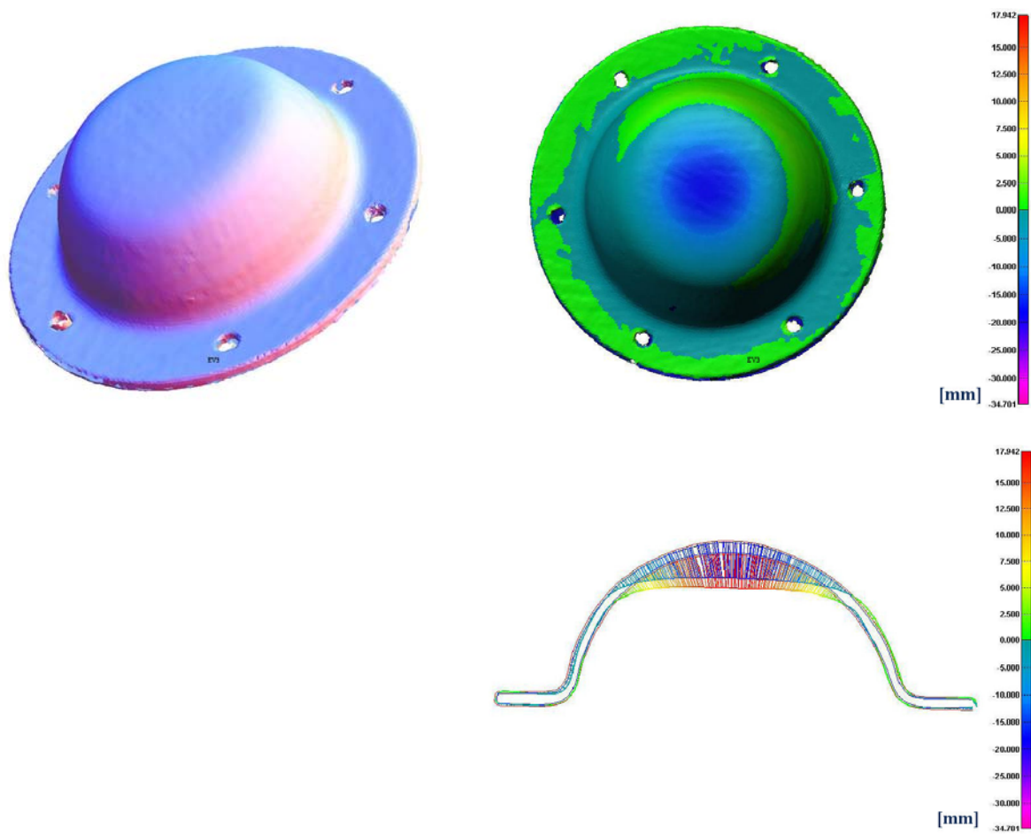
Figure B6. Nose: Full surface scan, contour map and cross-section
