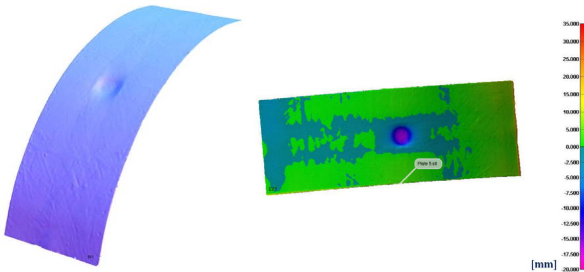
Figure B11. Dented Plate: Surface scan &amp; contour map
