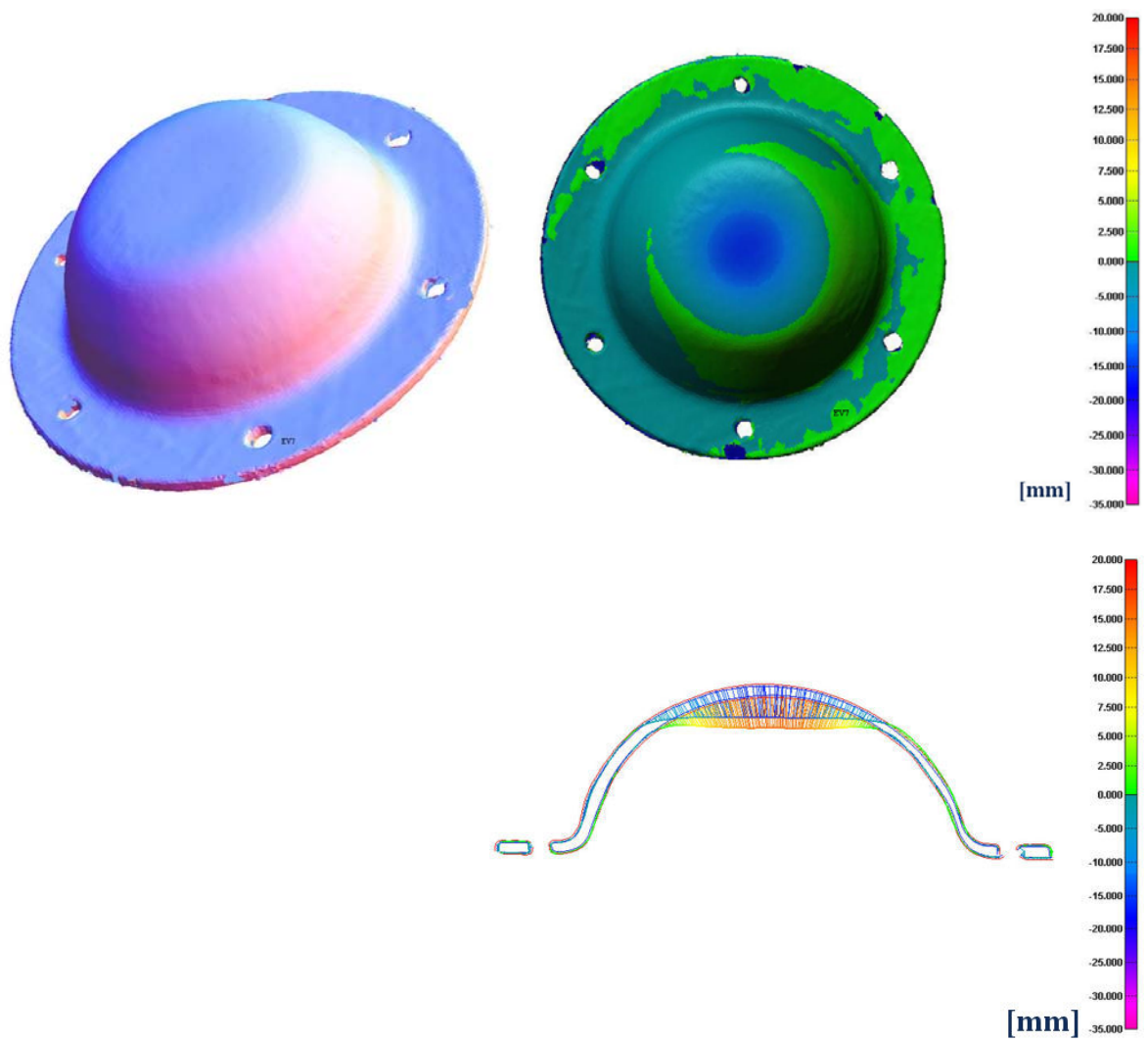
Figure B18. Nose: Full surface scan, contour map and cross-section
