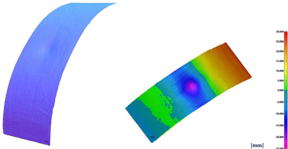
Figure B22. Dented Plate: Surface scan & contour map
