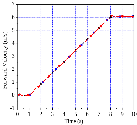
Figure 10: Chassis forward velocity
