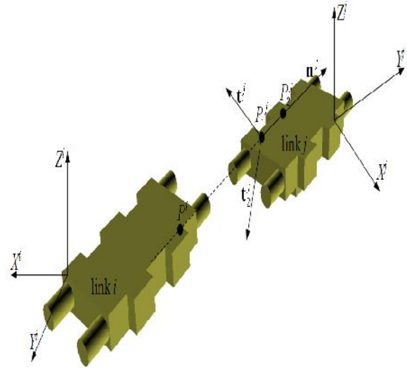
Figure 3: Bushing element
