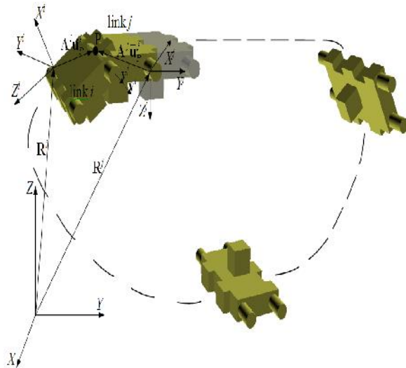
Figure 2: Revolute joint
