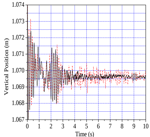
Figure 8: Chassis vertical displacement
