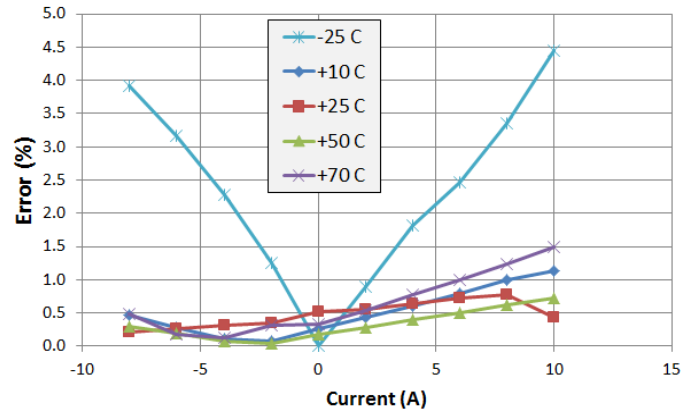
Figure 8. Error (%) of the MOSFET SSCB current sensor as a function of current and temperature. Positive current is current into the pack and out of the BMS.
