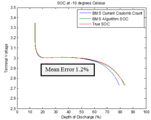
Figure 9. SOC measurements using the BMS prototype and pack at -10°C
