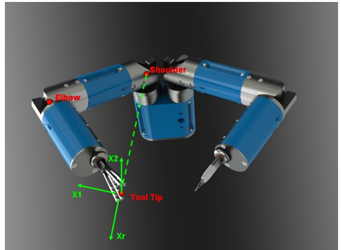
FIGURE 1. ROBOT DESIGN AND AXIS ORIENTATION
