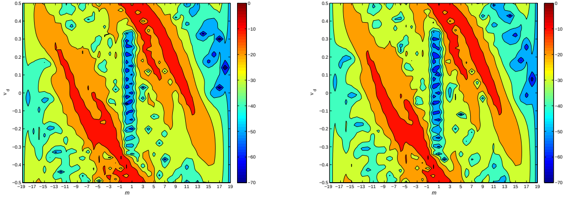
(c) Cross-Ambiguity Function of the radar code and receive filter (s^{(10)}, w^{(10)}) .
