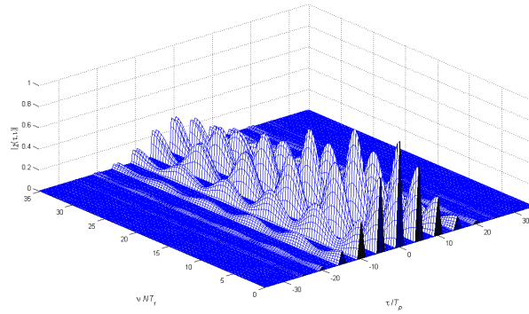
Figure 2.3: (a) Ambiguity function modulus of the designed code with N = 7 , T_r = 5T_p , \epsilon = 1.9998 and \gamma = 1 .
