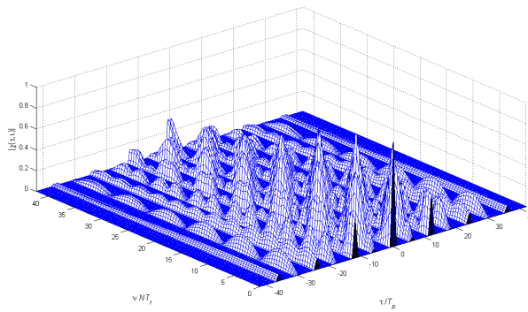
Figure 2.3: (b) Ambiguity function modulus of the designed code with N = 7 , T_r = 5T_p , \epsilon = 0.3 and \gamma = 1 .
