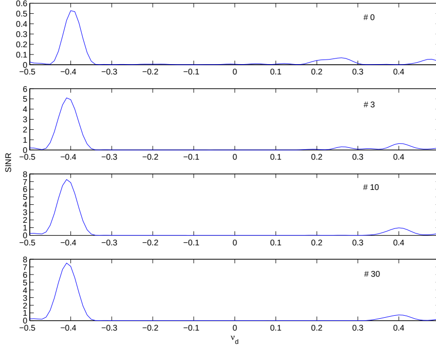
Figure 3.12: \text{SINR}^{(n)} versus the normalized Doppler \nu_d , for n = [0, 3, 10, 30] .
