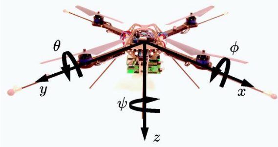
Flight Vehicle
