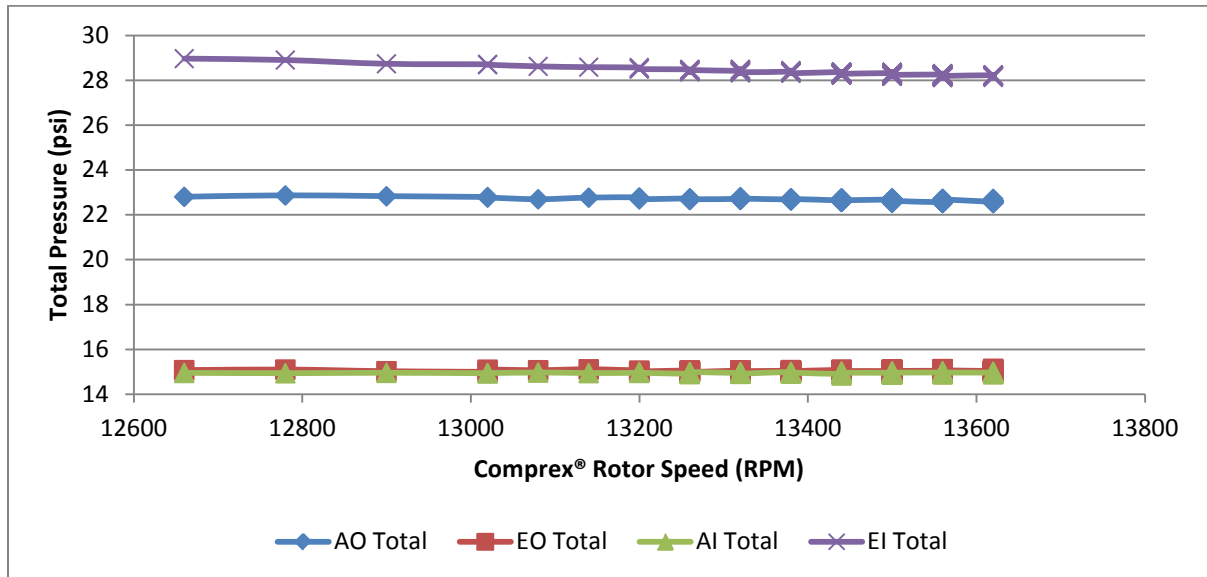
Figure 40: Total pressures in free running Compresx®, 15.9 lb/min at EI
