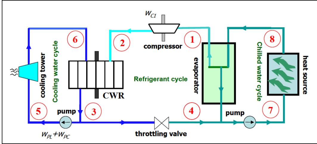
Figure 11: Schematic of R718 cooling unit enhanced by a condensing wave rotor (25)
