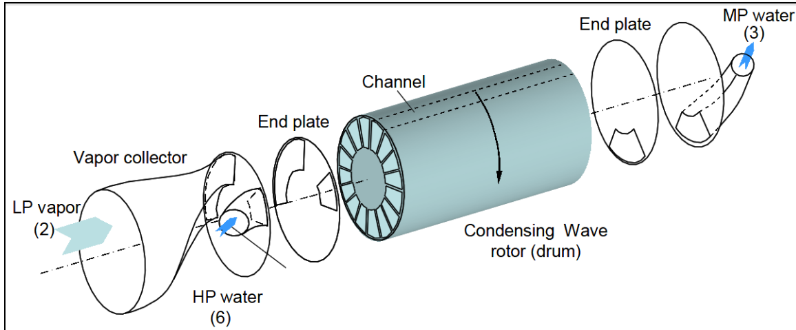
Figure 12: Schematic of three point condensing wave rotor (18)
