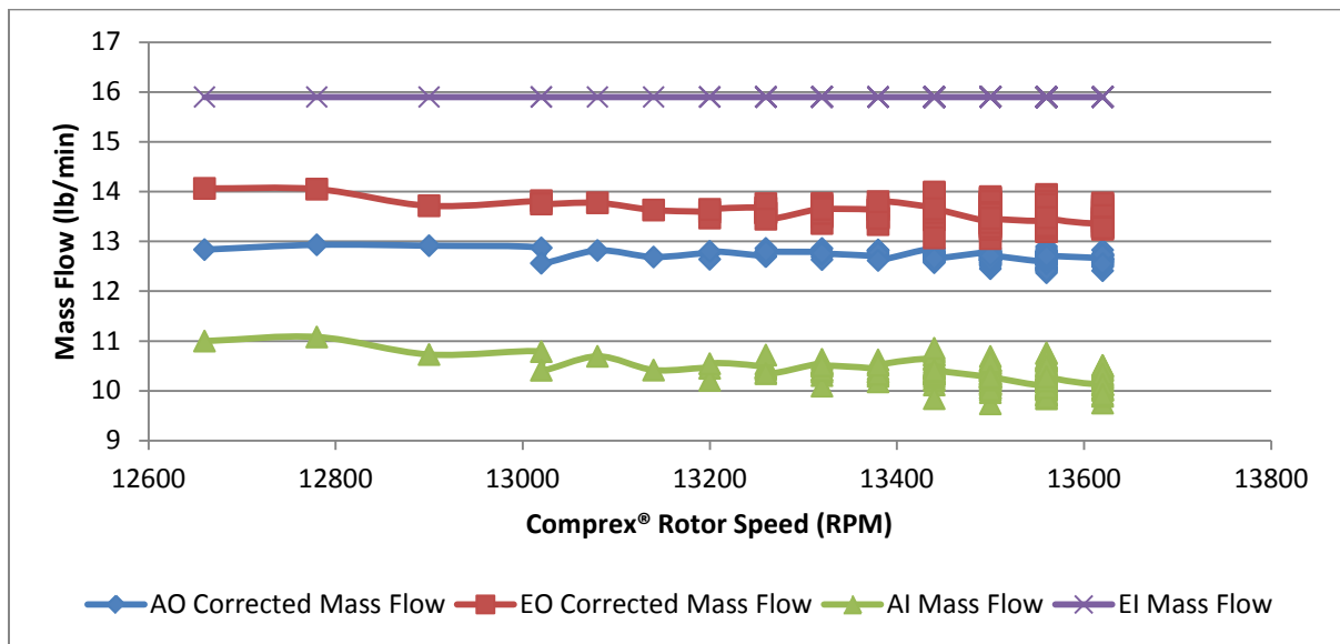
Figure 41: Mass flows in free running Compresx®, 15.9 lb/min at EI
