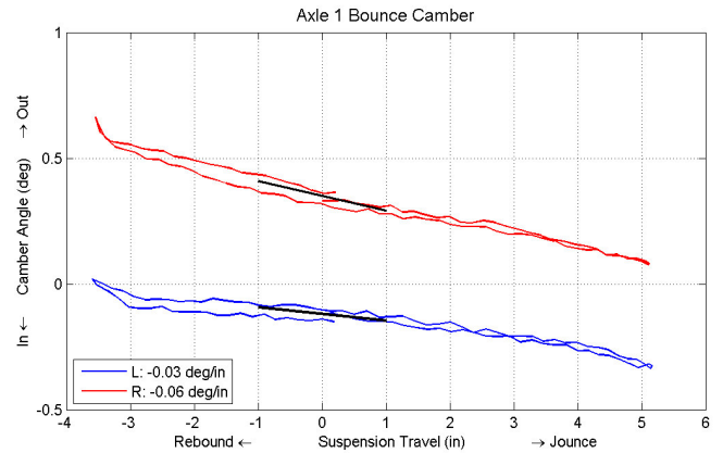
Figure 7: Bounce Camber Characteristic Curve
