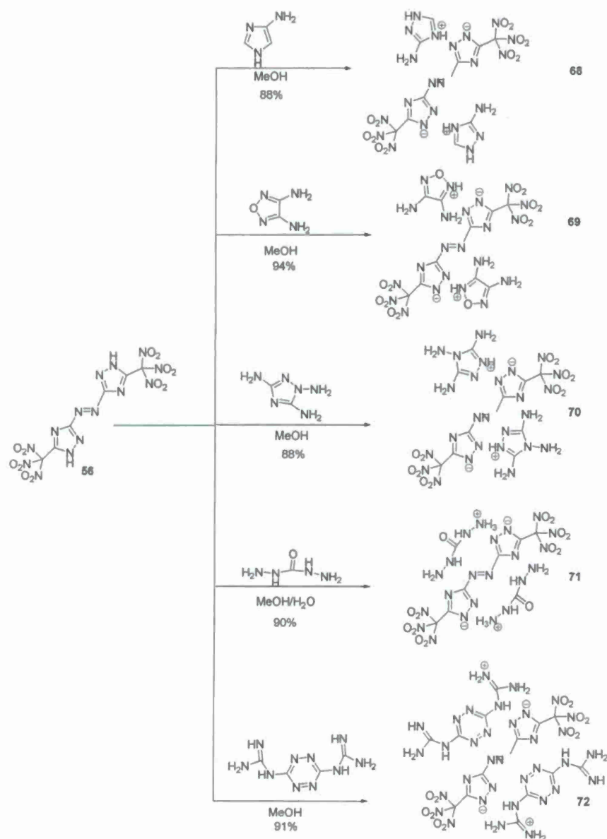
Scheme 17. Synthesis of energetic salts of 5,5'-bis(trinitromethyl)-3,3'-azo-1H-1,2,4-triazole (56).
