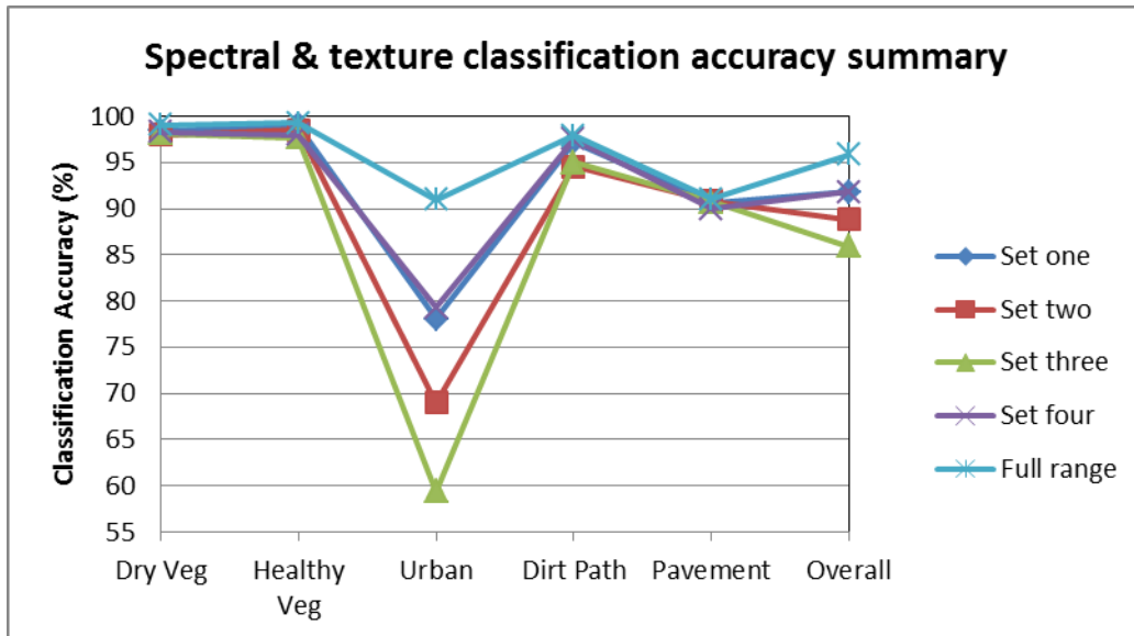
Figure 22. Spectral and texture classification accuracy summary.
