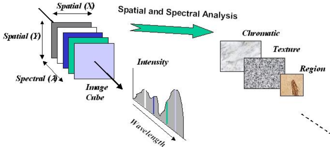
Figure 1. Hyperspectral imaging concept (From Chai et al., 2000).
