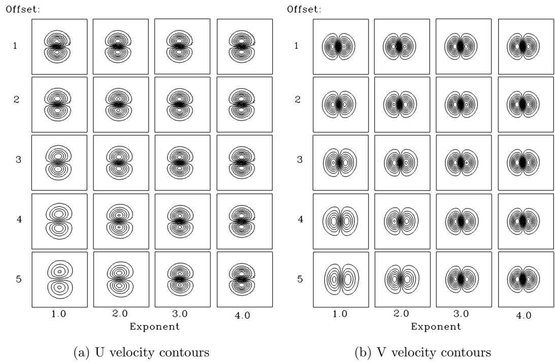
Figure 4.7: Velocity contours of the vortex C2F case parametric study of the IDW method
