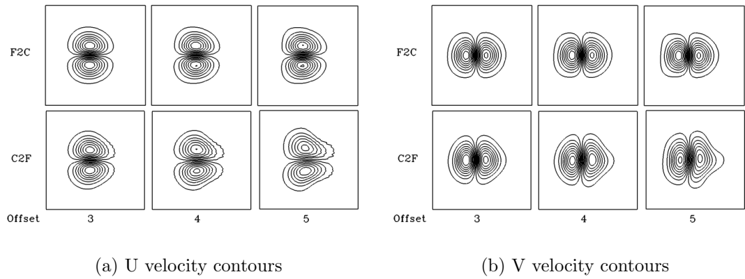
Figure 4.9: Velocity contours of the vortex case parametric study of the MLS method
