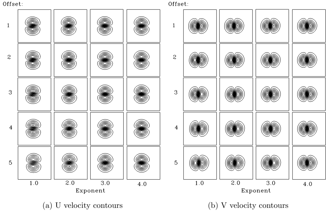
Figure 4.8: Velocity contours of the vortex F2C case parametric study of the IDW method
