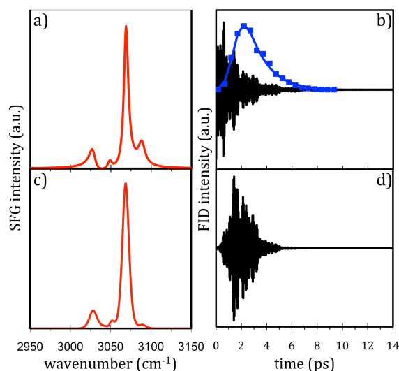
Figure 3. a) Simulated resonant spectrum with b) corresponding free induction decay (FID). The measured time profile of the visible pulse is also shown in b). Delay of the visible pulse c) alters the spectrum by d) apodizing the resonant FID. From Reference 4.
