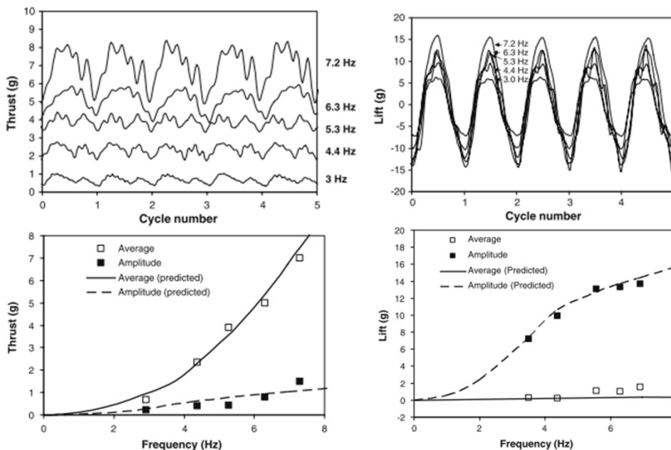
(top) Cyclic Variation of Lift and Thrust, (bottom) Variation with Flapping Frequency
