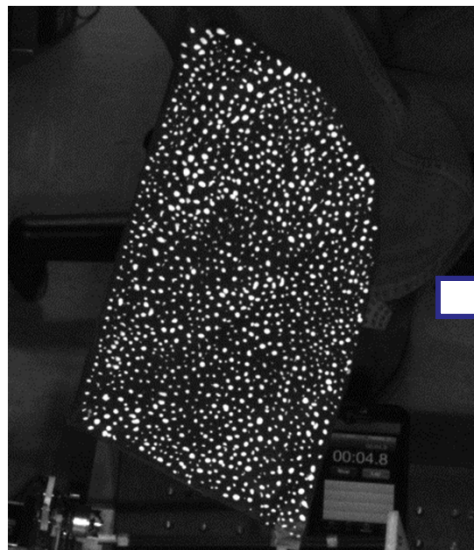
Wing w/speckle pattern for DIC
