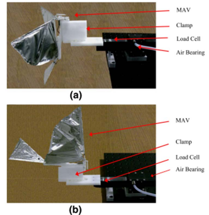
Test Stand for Measuring: (a) Lift & (b) Thrust
