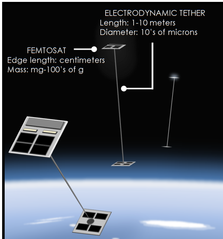
Concept of ED tethers with pairs of femtosats as a maneuverable and coordinated fleet
