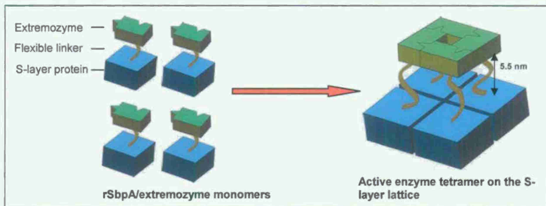
Fig. 19. Schematic drawing of the construction of S-layer-based biocatalysts carrying multimeric extremozymes. The active enzyme is formed by self-assembly of four monomeric subunits of the S-layer/extremozone fusion protein.
