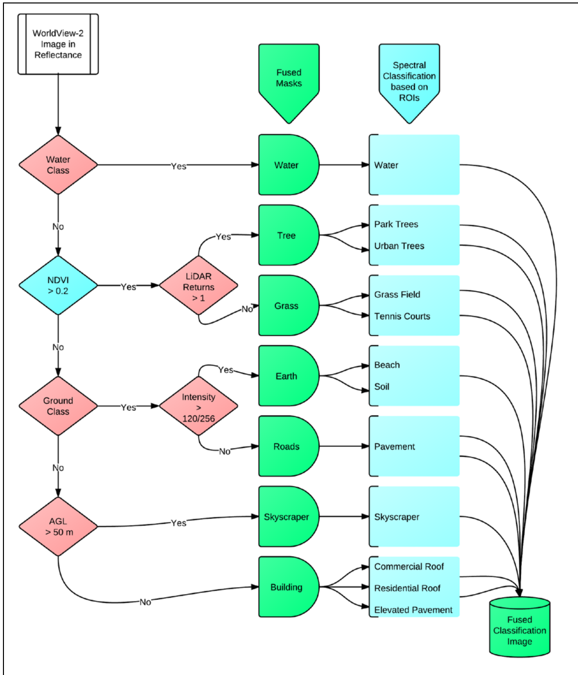
Figure 38. Flowchart of fusion classification technique decision tree
