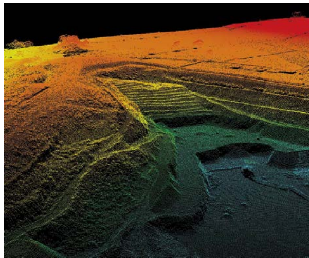
Figure 2. Example of a point cloud after processing and colored by height (From Cambridge University, 2006)
