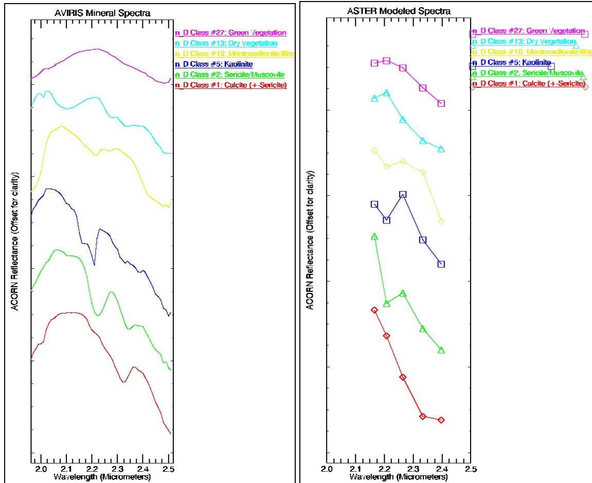
Figure 5. Comparison of AVIRIS (left) hyperspectral spectra and ASTER (right) multispectral spectra for selected minerals, dry, and green vegetation (From Kruse, 2007).
