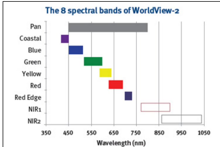
Figure 12. The wavelength ranges of WorldView-2 (From DigitalGlobe, 2011)
