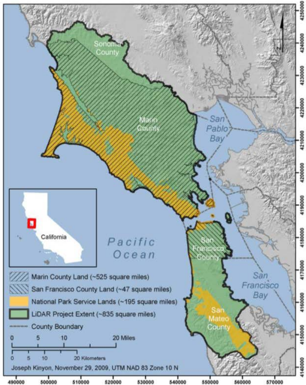
Figure 21. Golden Gate LiDAR Project acquisition area (From Hines, 2009)
