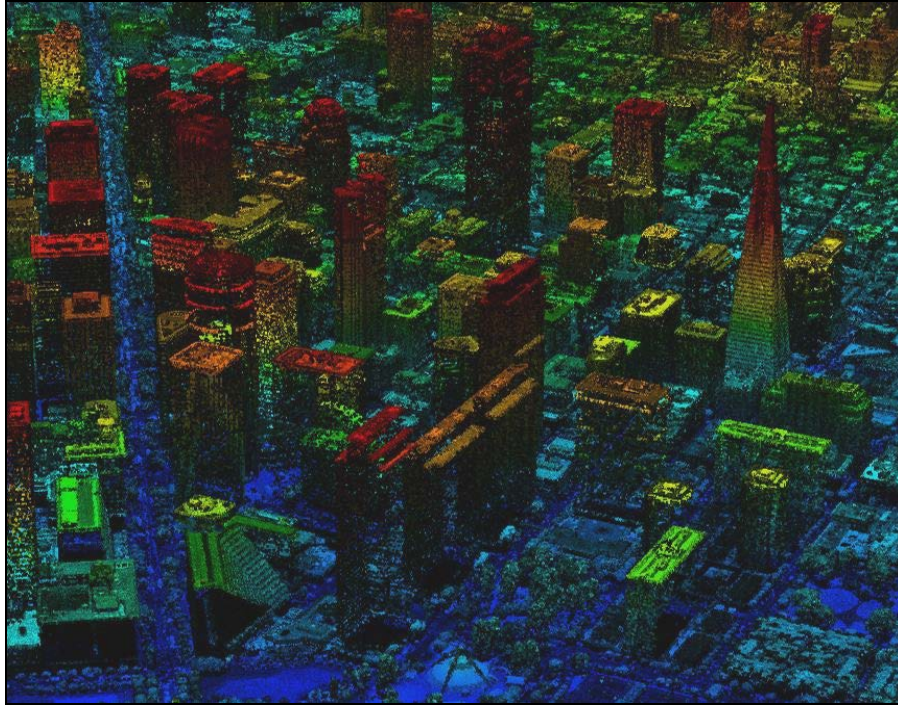
Figure 22. A sample of the GGLP point cloud over downtown San Francisco viewed in Quick Terrain Modeler
