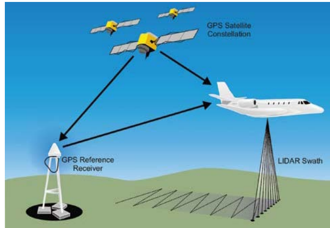
Figure 1. LiDAR data flow in an airborne system (From Holden et al., 2002)
