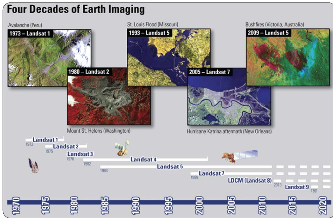
Figure 6. Landsat timeline and imaging samples (From USGS, 2012)
