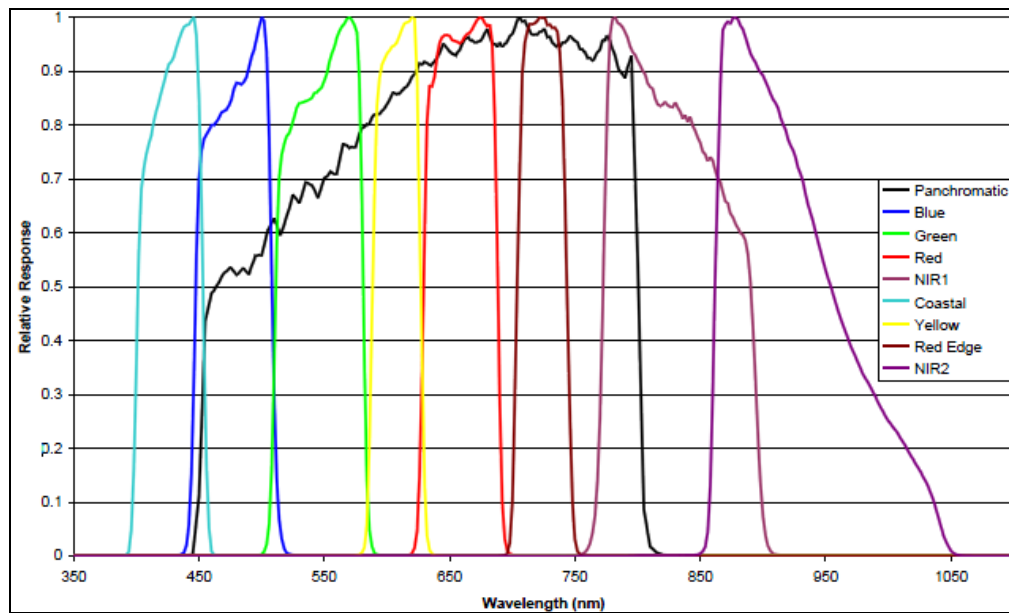
Figure 13. The Relative Spectral Radiance Response of WorldView-2 (From DigitalGlobe, 2011)
