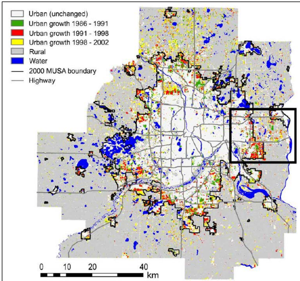
Figure 8. Land cover changes from Landsat in the Twin Cities from 1986 to 2002 (From Yuan et al., 2005)
