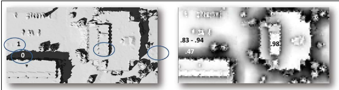
Figure 16. Shadow map (left) and an illumination map (right) created from LiDAR images at the Rochester Institute of Technology (From Ientilucci, 2012)
