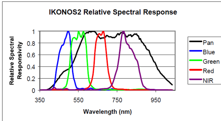
Figure 9. IKONOS spectral response bands (From Dial & Grodecki, 2003).
