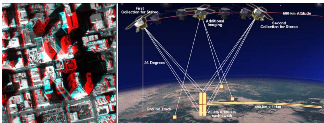
Figure 10. An example of an IKONOS visualization of a stereo pair and the satellite pass to obtain it (From Dial & Grodecki, 2003).
