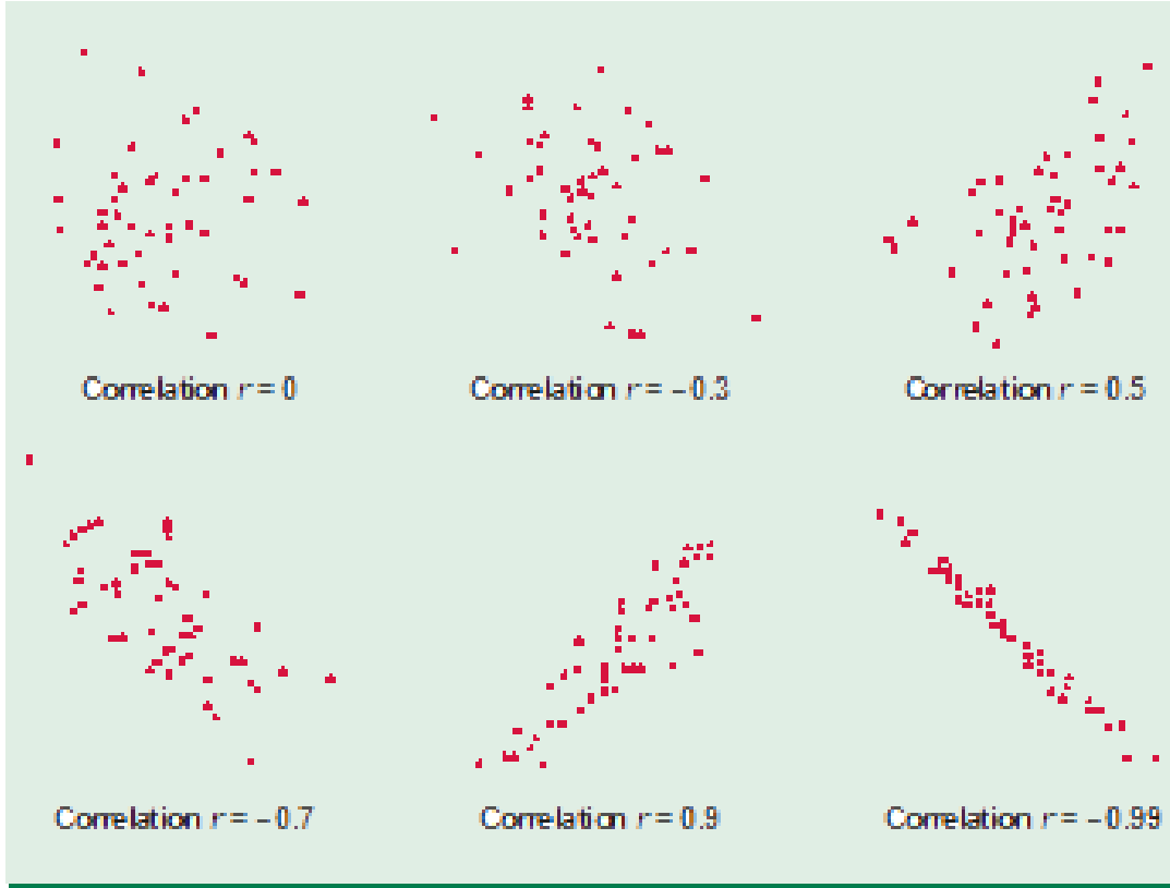
Figure 1. Example of how correlation measures the direction and strength of a linear relationship. From Moore et al. (2011)
