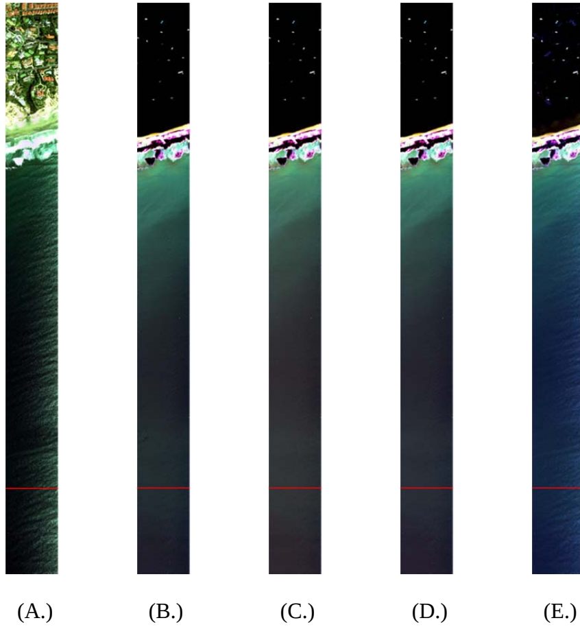
Figure 14. True-color composite depictions of the hyperspectral test image (A.), and sun glint corrected images from the methods of Hedley et al. (B.), Lyzenga et al. (C.), Joyce (D.), and Kuster et al. (E.). Blue represents the (456–464 nm) band, green represents the (548–555 nm) band, and red represents the (637–645 nm) band. The red lines represent the deep water ROI pixel locations of (1–320, 3000).
