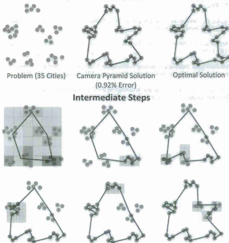
Figure 12. Top row: the problem, its solution by the limited memory model and the optimal solution. The next two rows illustrate the solution process. The process begins with 5 clusters coded by different colors. One of the clusters (bottom right) is chosen as the starting cluster. Then, the solution proceeds clockwise.
